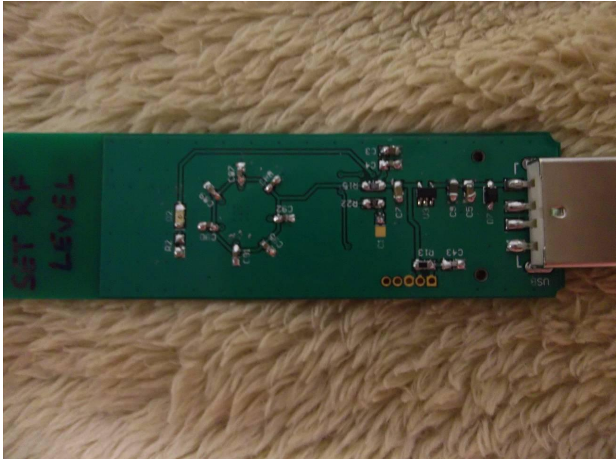
Figure 2. Bottom of PCB
