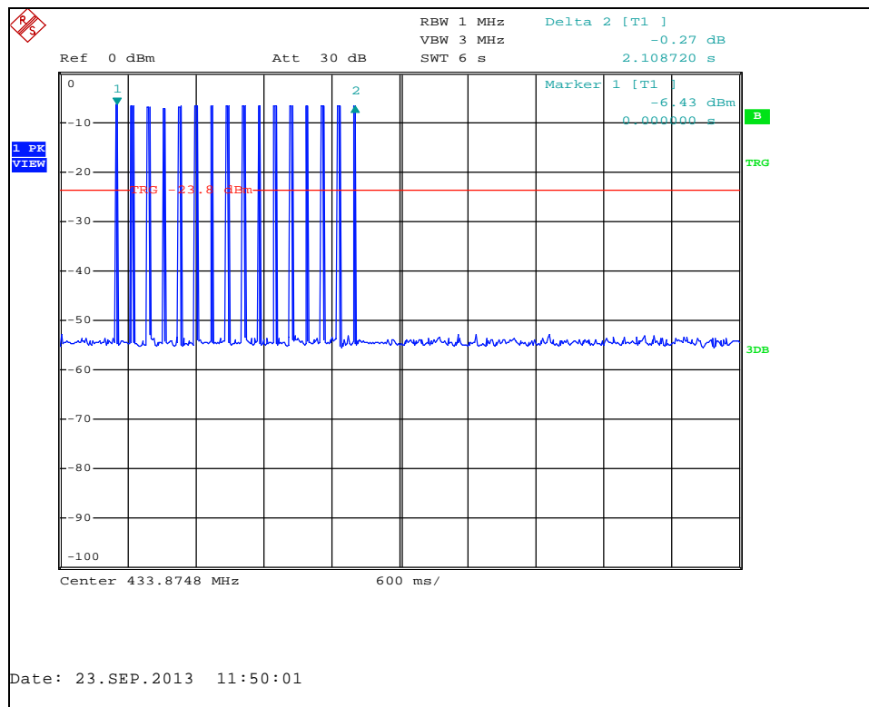
Figure 7.3.2-2: TX Hold Time – FSK Modulation
