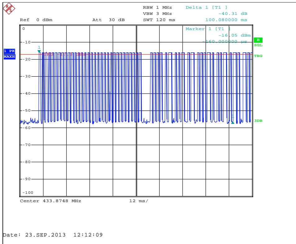
Figure 7.5.2-2: Duty Cycle - 100ms Period - ASK Modulation
