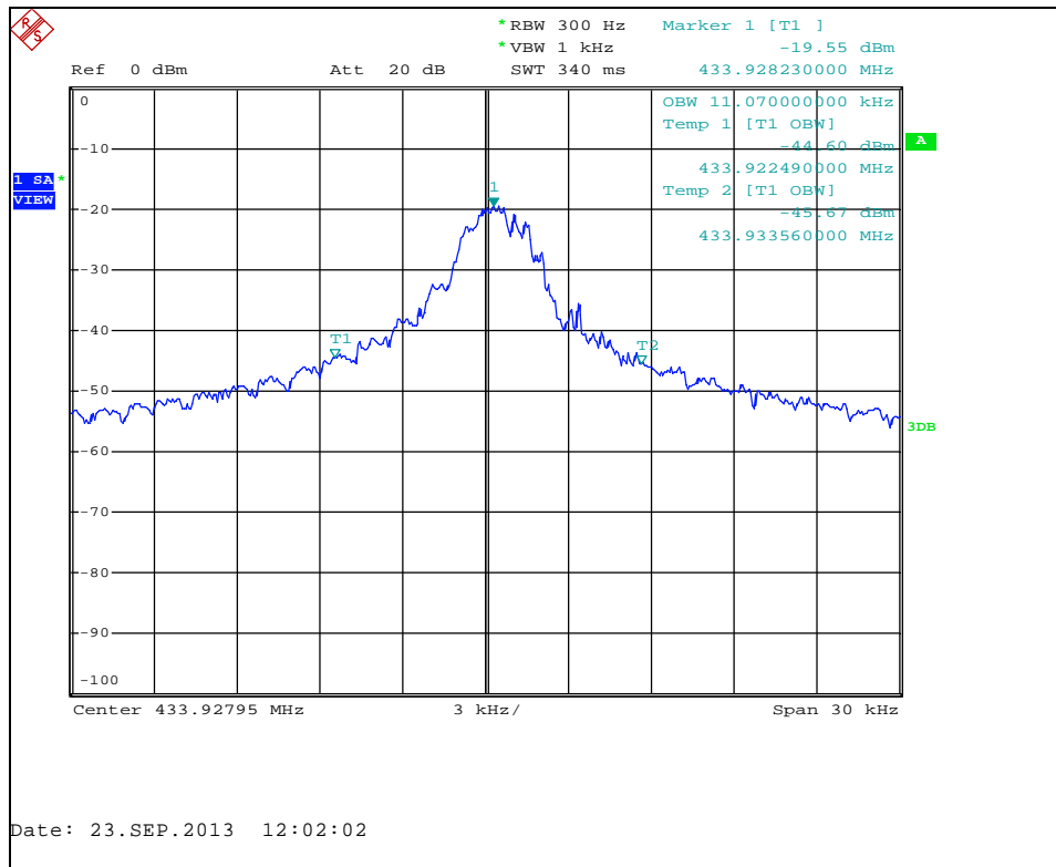
Figure 7.4.2-2: 99% Occupied Bandwidth – ASK Modulation
