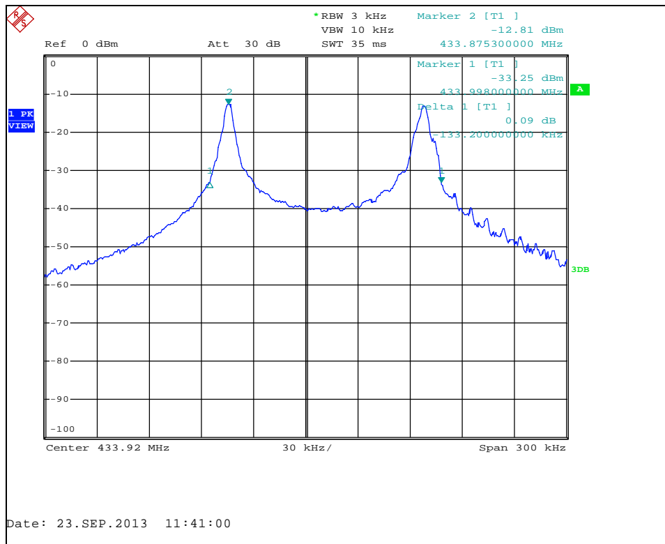
Figure 7.4.2-3: 20 dB Bandwidth – FSK Modulation
