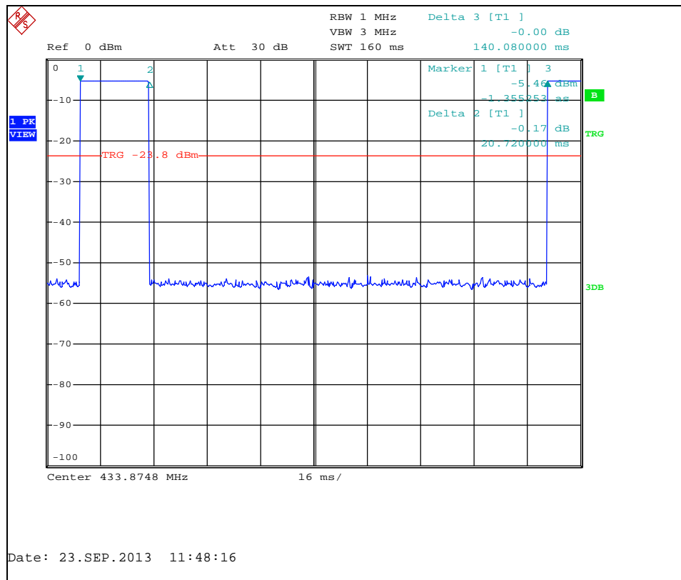
Figure 7.5.2-5: Duty Cycle – FSK Modulation
