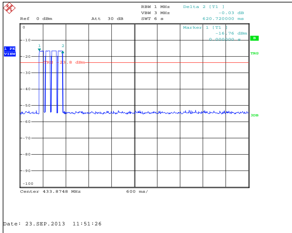
Figure 7.3.2-1: TX Hold Time – ASK Modulation
