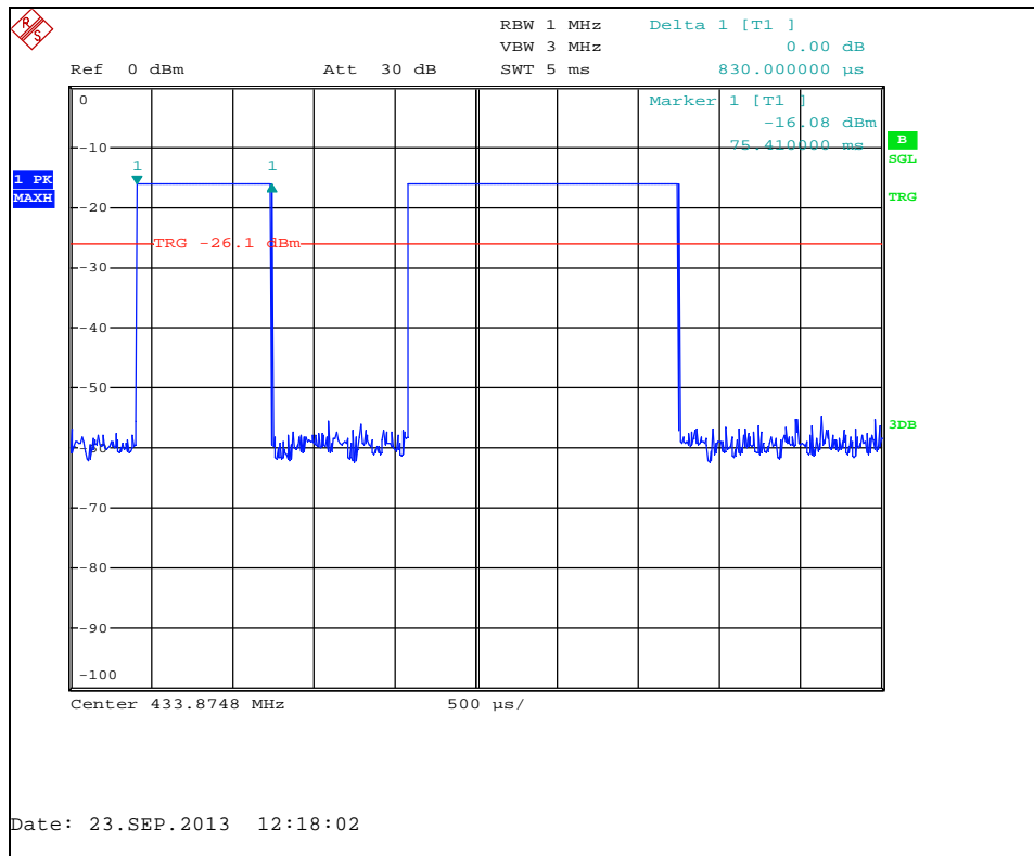
Figure 7.5.2-3: Duty Cycle –Pulse Width (T1) - ASK Modulation
