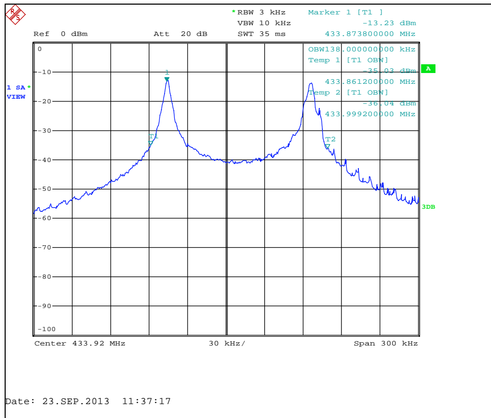
Figure 7.4.2-4: 99% Occupied Bandwidth – FSK Modulation
