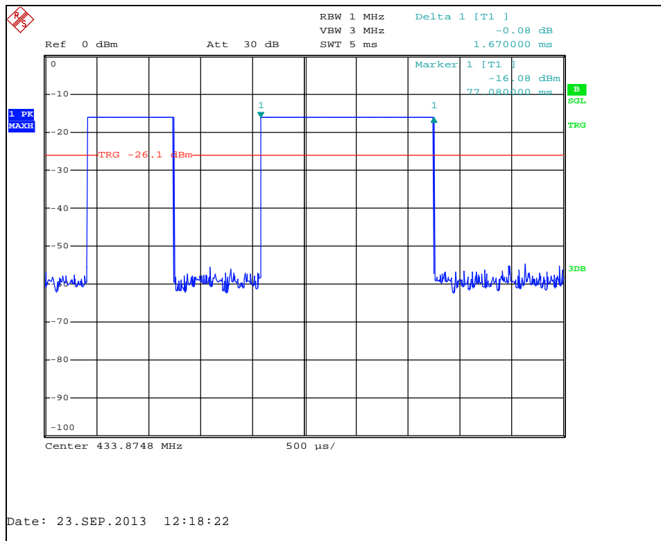
Figure 7.5.2-4: Duty Cycle – Pulse Width (T2) - ASK Modulation
