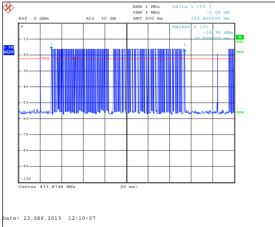
Figure 7.5.2-1: Pulse Train Period – ASK Modulation
