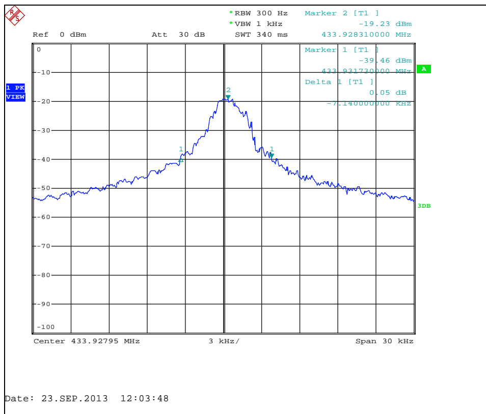
Figure 7.4.2-1: 20 dB Bandwidth – ASK Modulation
