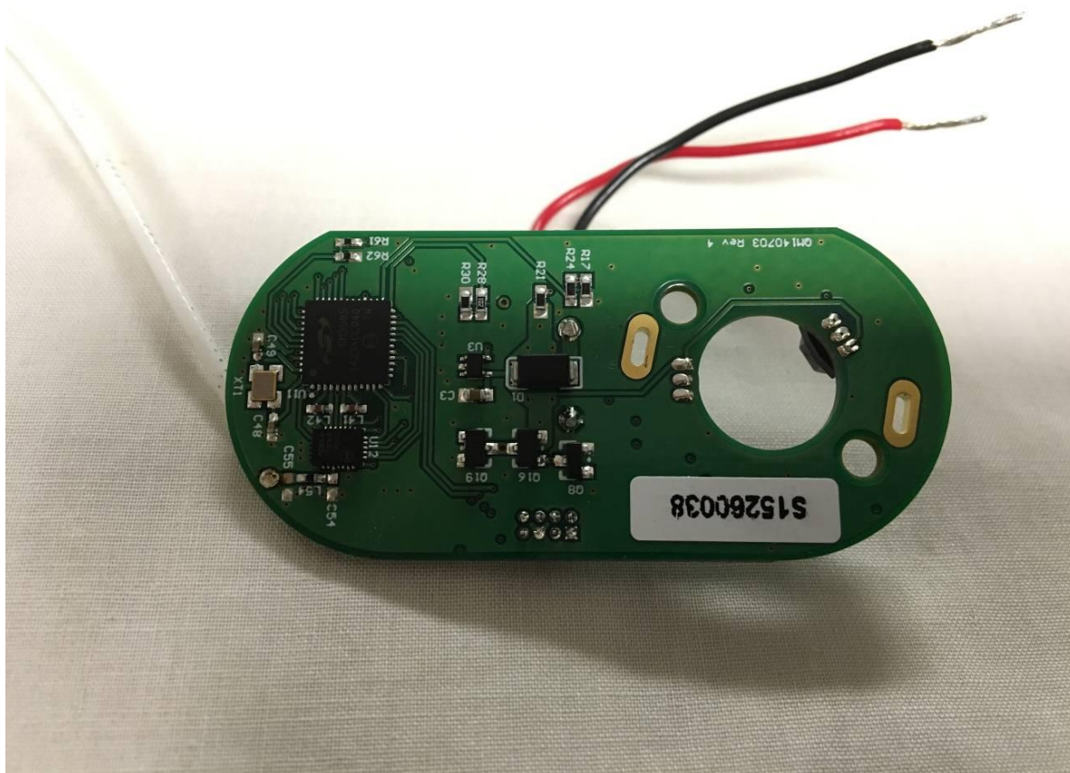
Figure 9. PCB Side 1
