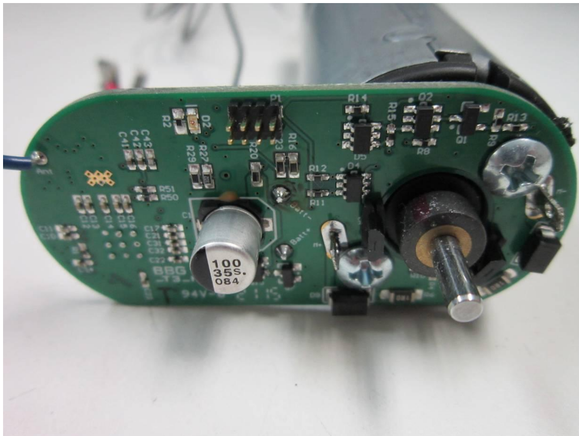
Figure 7. PCB Mounted to Motor
