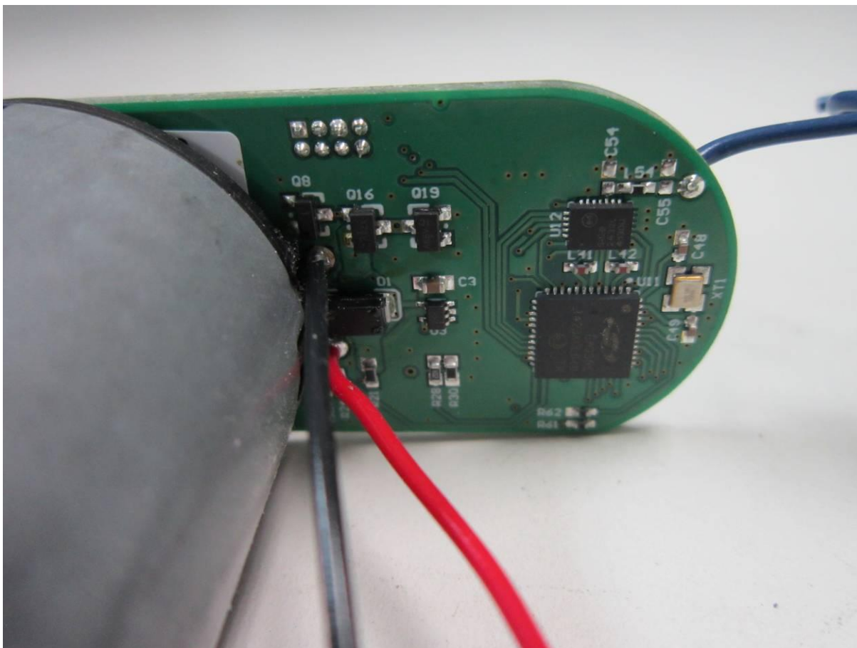
Figure 8. PCB Mounted to Motor
