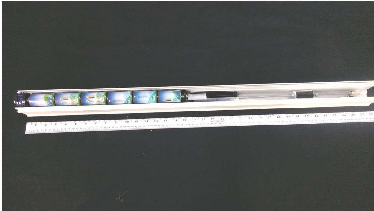
Figure 1. Facia Removed (EUT/Motor Exposed)
