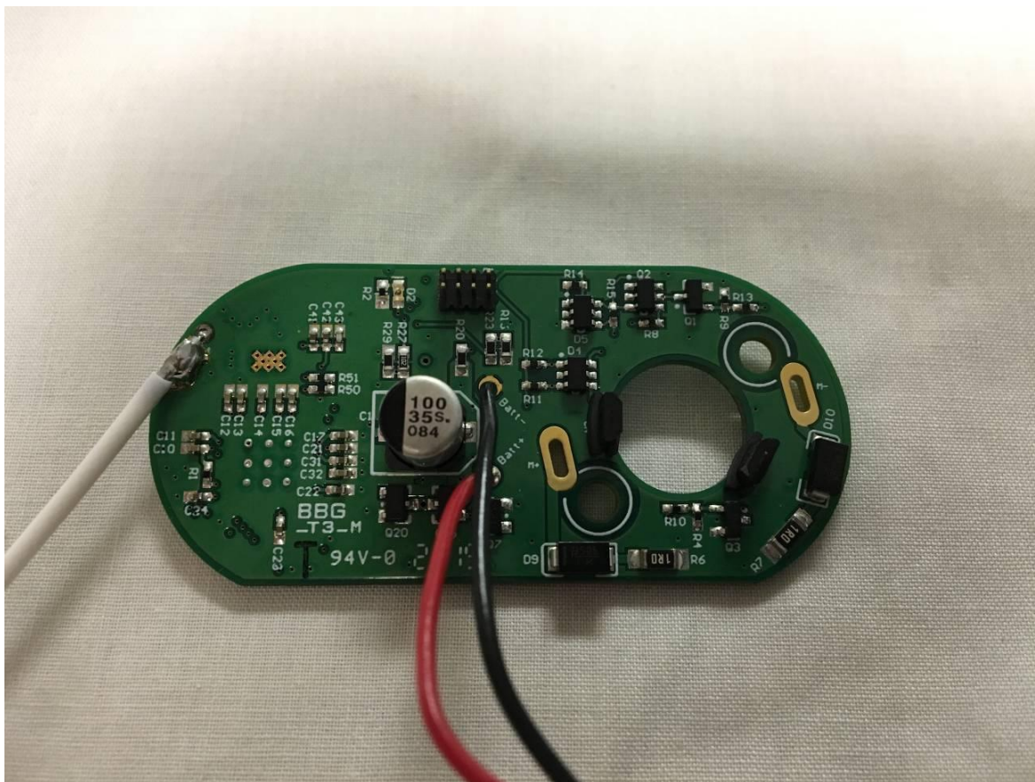
Figure 10. PCB Side 2
