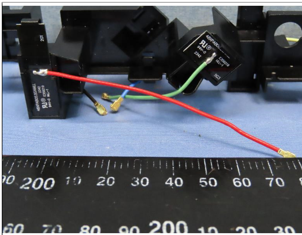
2G1 Antenna
