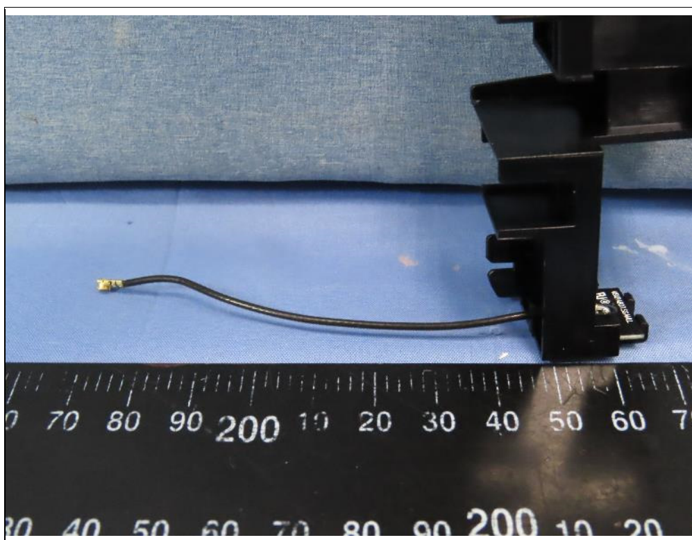
5G1 Antenna
