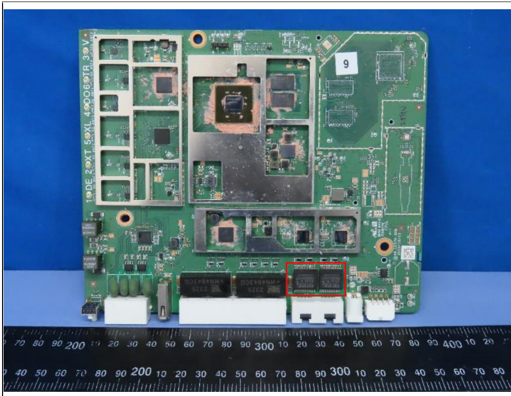
2 nd Transformer
