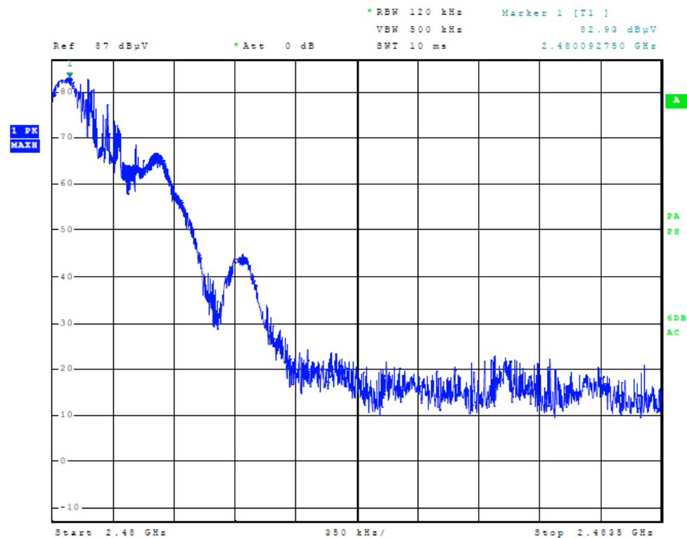
Figure 10 Plot of Transmitter High Band Edge
