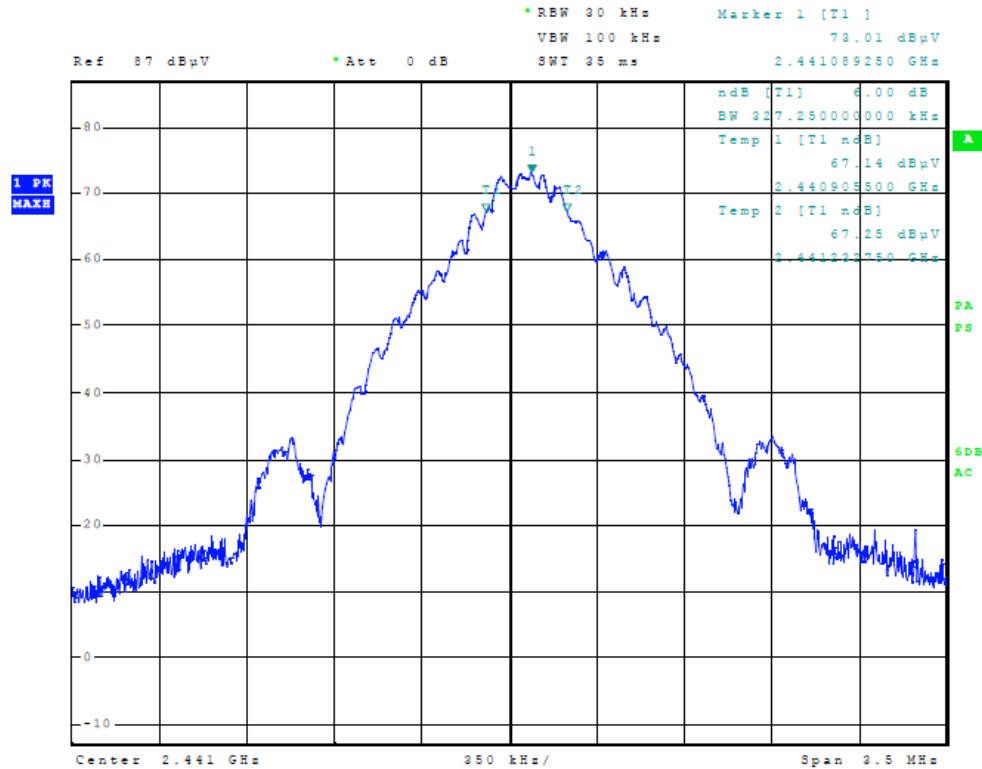
Figure 5 Plot of Transmitter Occupied Bandwidth (6-dB)
