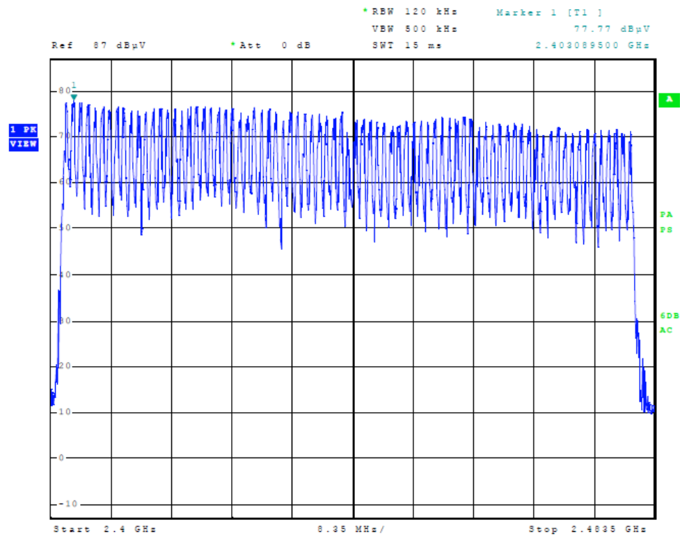
Figure 3 Plot of Transmitter Emissions in Operational Frequency (number of Hops)
