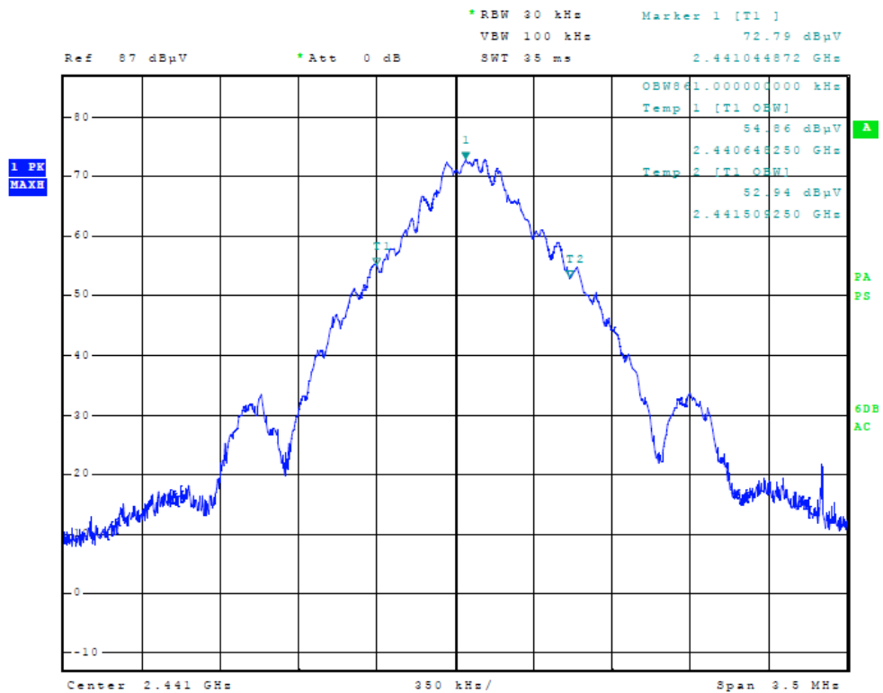
Figure 6 Plot of Transmitter Occupied Bandwidth (99.5 percent)
