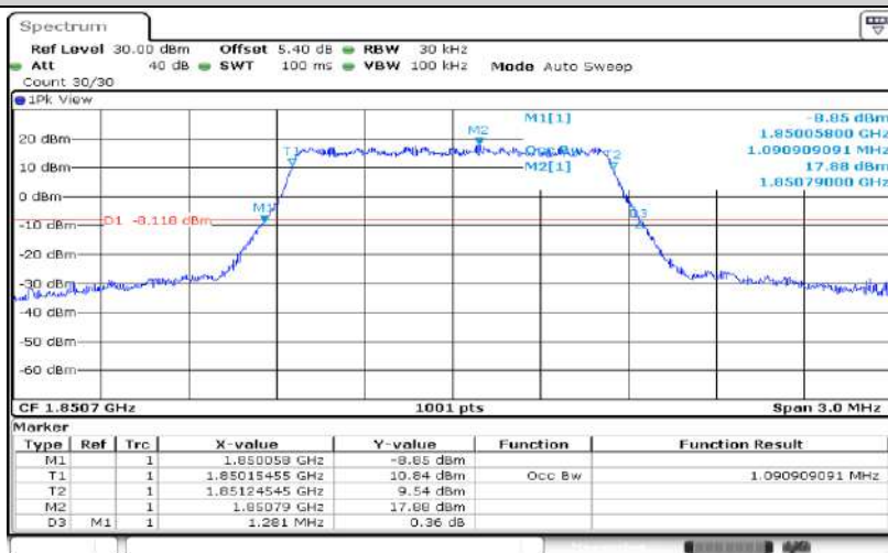
Band2-1.4MHz-QPSK-18607-6RB#0-1.091
