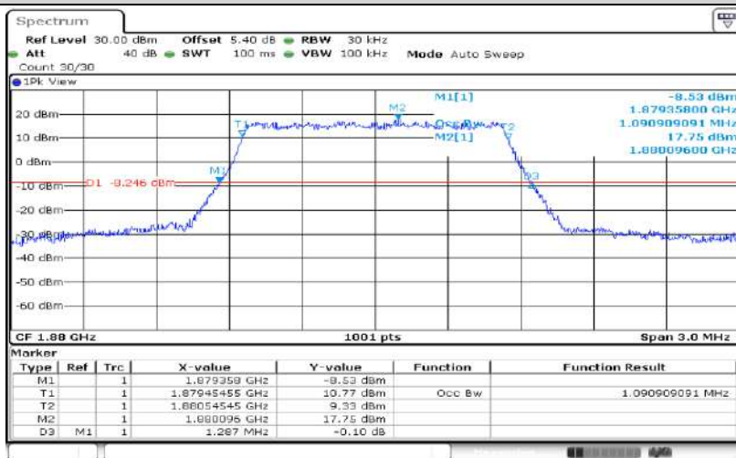
Band2-1.4MHz-QPSK-18900-6RB#0-1.091
