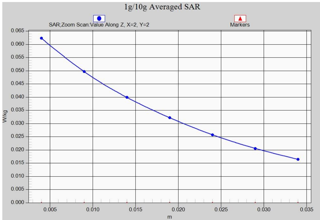
Fig.17-1 Z-Scan at power reference point
