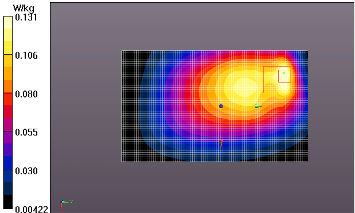
Fig.18 LTE Band 17
