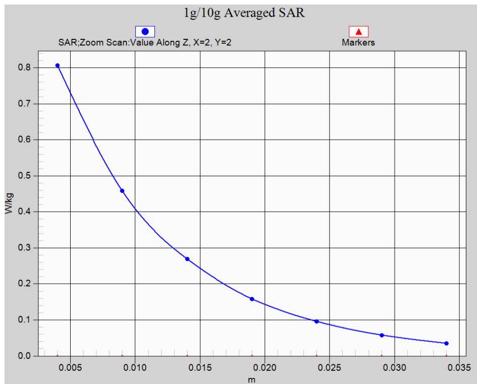
Fig.12-1 Z-Scan at power reference point (Band 2 CH19100)
