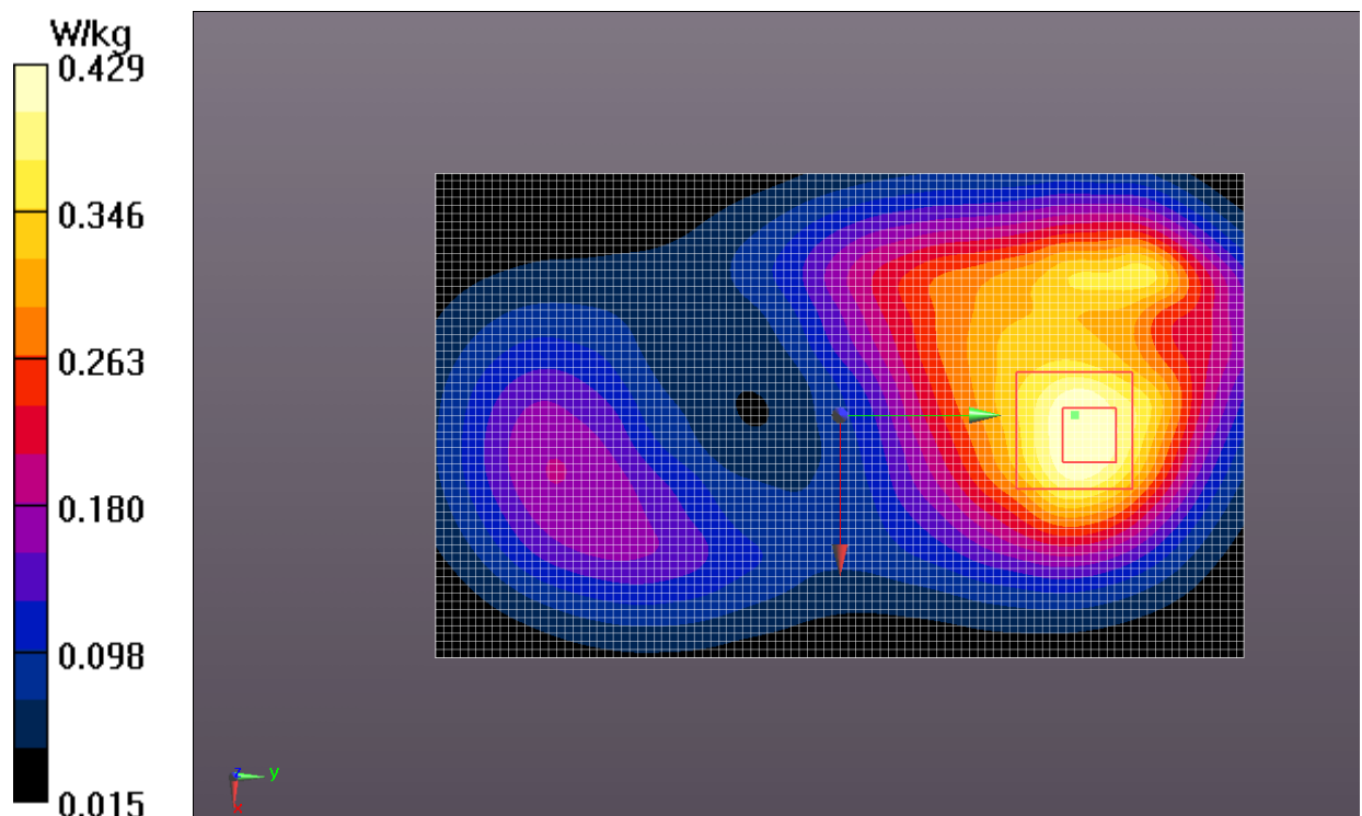
Fig.12 LTE Band 2 CH19100
