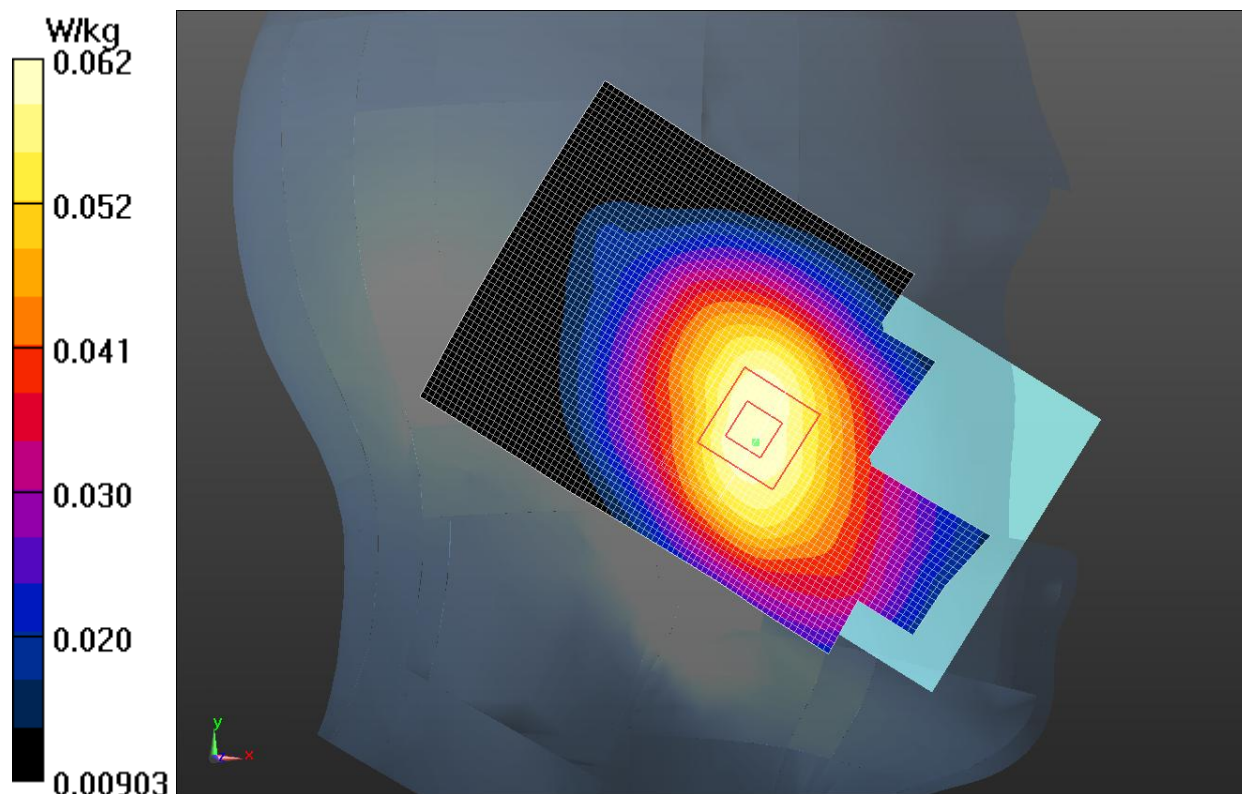
Fig.17 LTE Band 17
