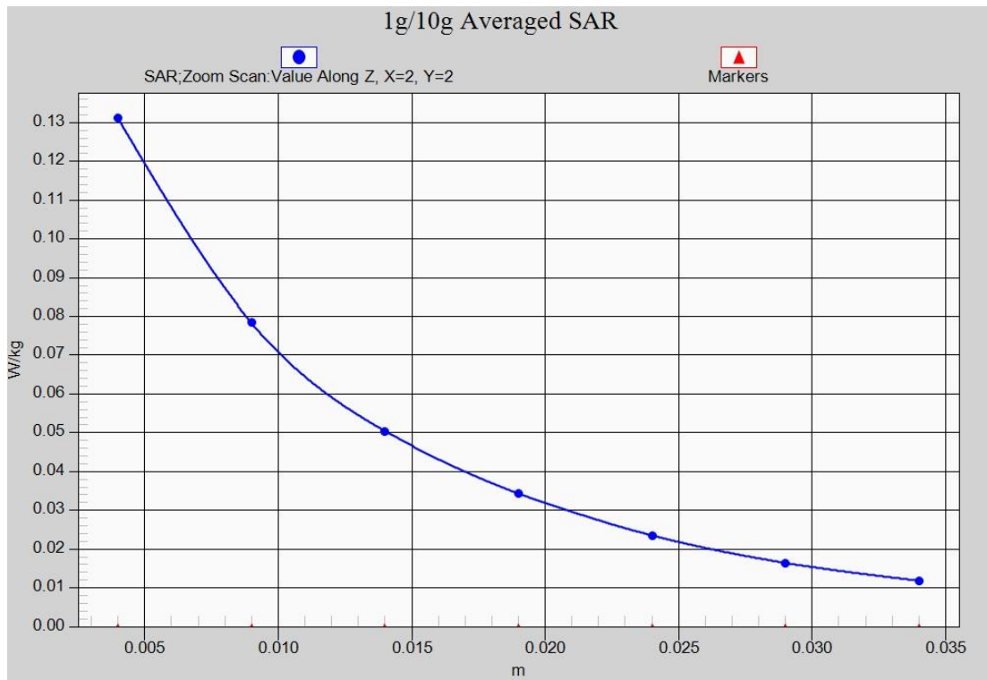
Fig.18-1 Z-Scan at power reference point (Band 17 )
