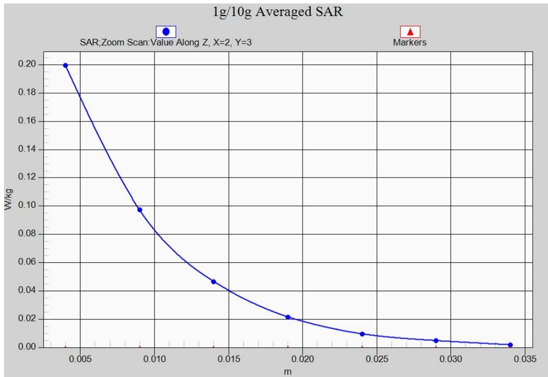
Fig.19-1 Z-Scan at power reference point (Wi-Fi 2450 MHz CH6)
