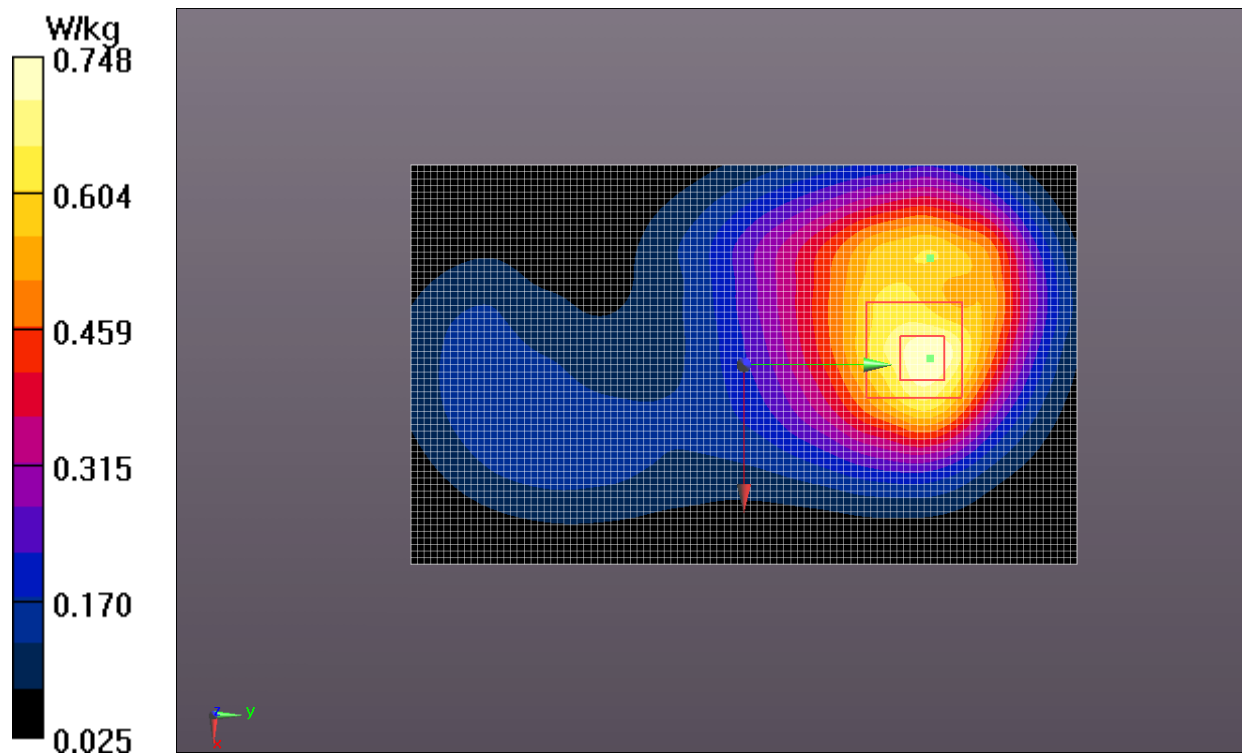
Fig.14 LTE Band 4 CH20300
