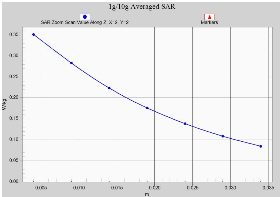
Fig.16-1 Z-Scan at power reference point (Band 5)
