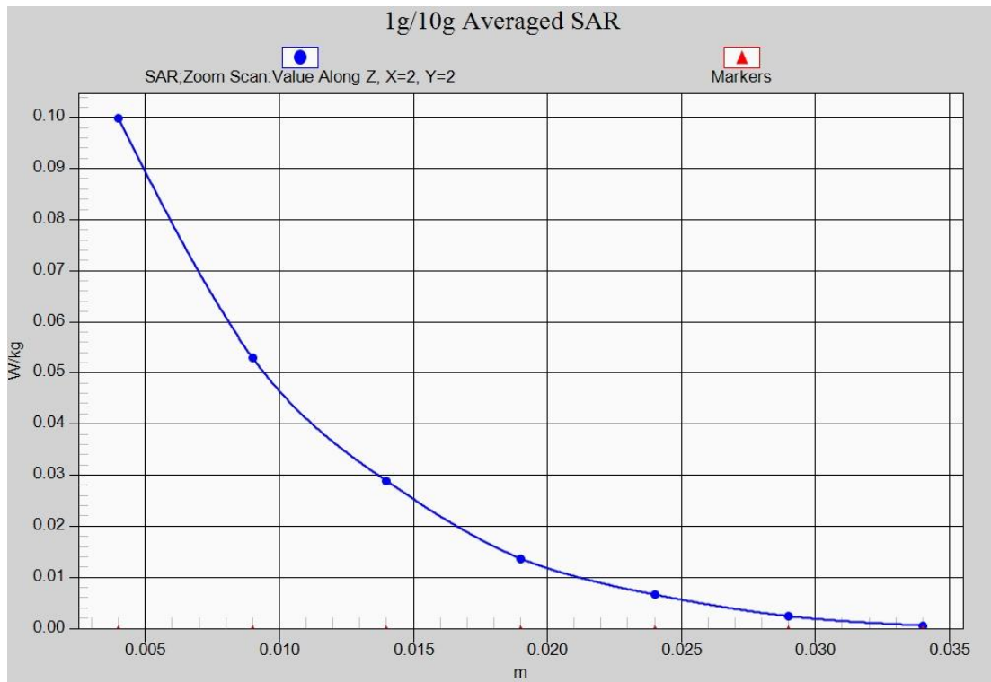
Fig.20-1 Z-Scan at power reference point (Wi-Fi 2450 MHz CH6)
