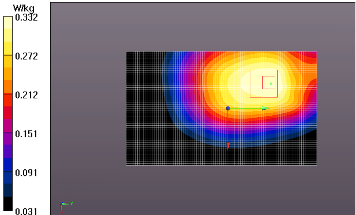
Fig.16 LTE Band 5
