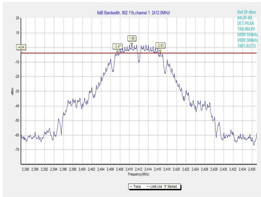
Fig.A.4.1 Occupied 6dB Bandwidth(802.11b,Ch 1)
