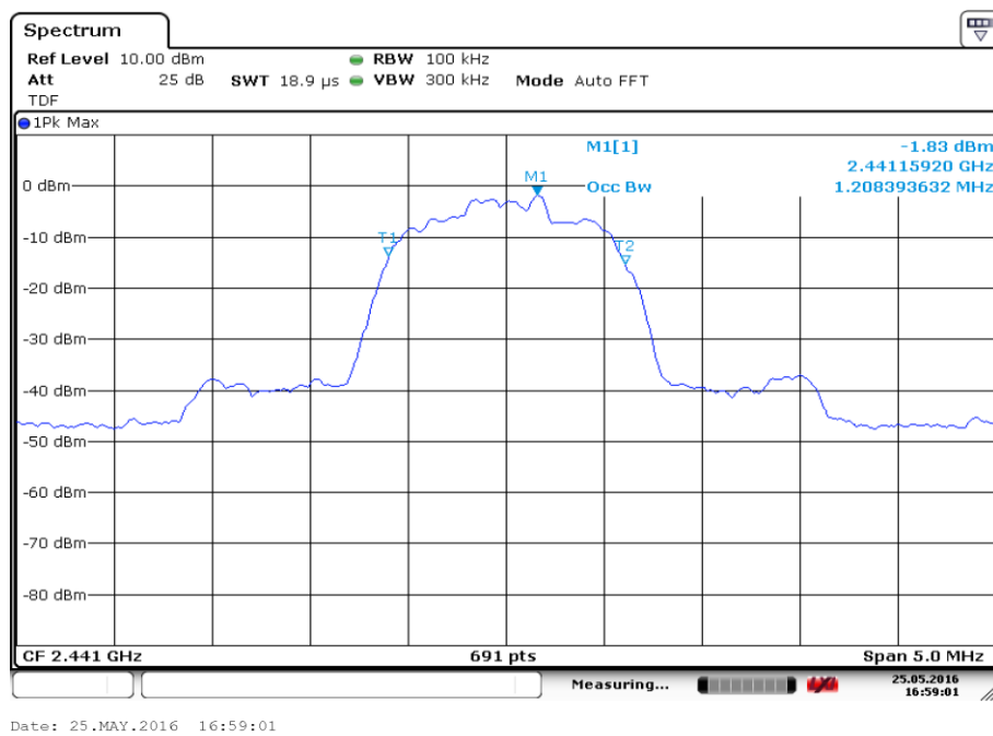
Fig.94. Occupied Bandwidth: 8DPSK, Channel 39
