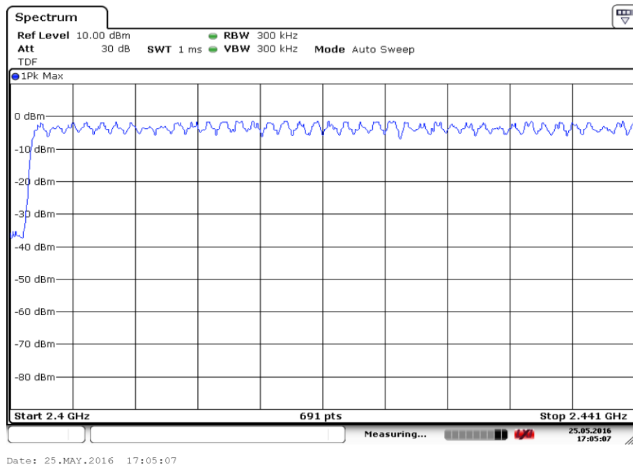
Fig.83. Number of hopping frequencies: \pi/4 DQPSK, Channel 0 - 39
