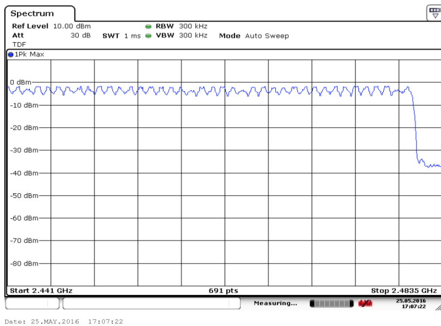
Fig.84. Number of hopping frequencies: \pi/4 DQPSK, Channel 40 - 78
