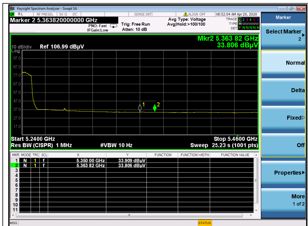
(AVG,Channel48,802.11n (HT20))
