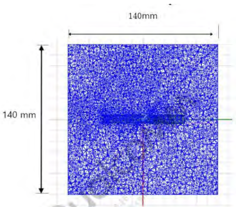
Figure 1-1: Example of HFSS mesh in a model of the device (Top view)
