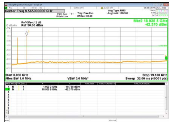
B13_N2(10M)_DFT-s-OFDM_QPSK_Edge_1R B_Left_High_CH
