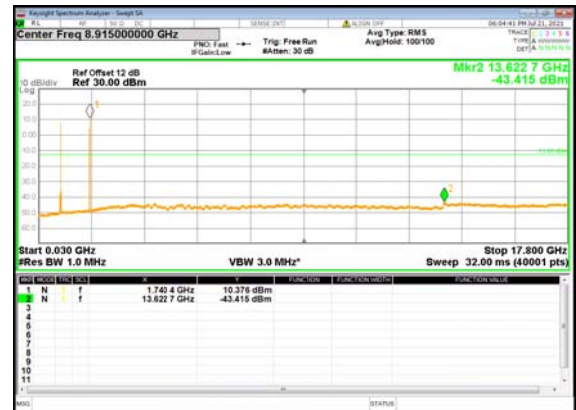
B13_N66(10M)_DFT-s-OFDM_QPSK_Edge_1 RB_Left_Mid_CH
