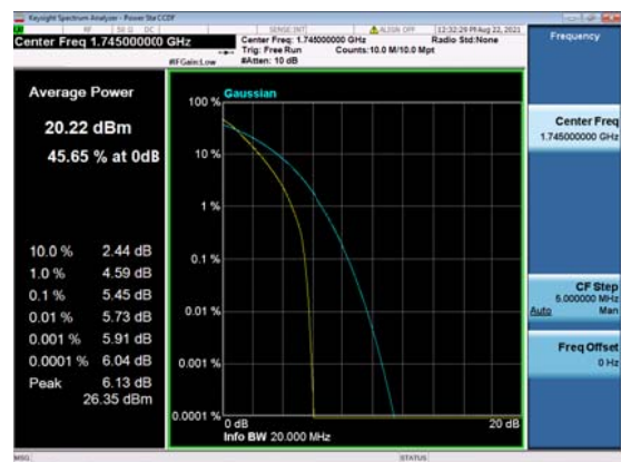
B13_N66(20M)_DFT-s-OFDM_QPSK_Outer_Full_Mid_CH
