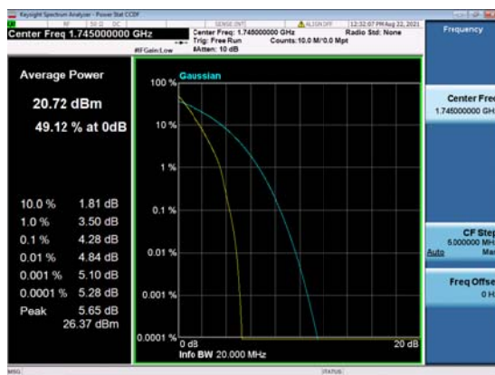
B13_N66(20M)_DFT-s-OFDM_PI_2-BPSK_Outer_Full_Mid_CH
