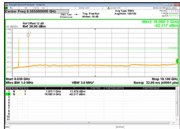
B13_N2(15M)_DFT-s-OFDM_QPSK_Edge_1R B_Left_Mid_CH
