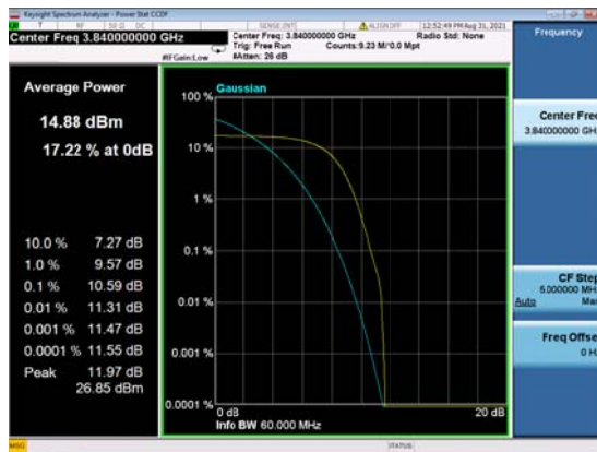
B5_N77(60M)_DFT-s-OFDM_PI_2-BPSK_Outer_Full_Mid_CH
