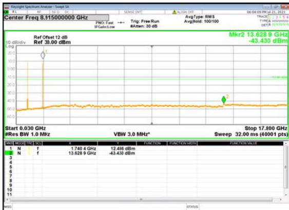
B13_N66(10M)_DFT-s-OFDM_BPSK_Edge_1 RB_Left_Mid_CH
