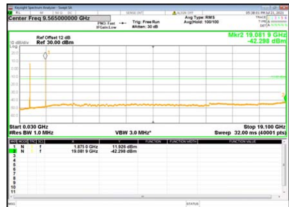
B13_N2(10M)_DFT-s-OFDM_QPSK_Edge_1R B_Left_Mid_CH
