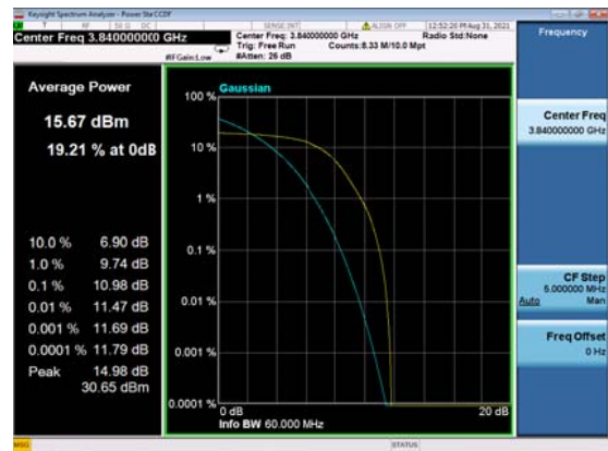
B5_N77(60M)_DFT-s-OFDM_QPSK_Outer_Full_Mid_CH
