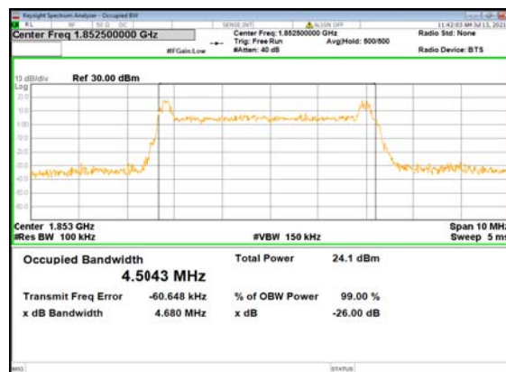
N2(5M)_DFT-s-OFDM_64QAM_Outer_Full_Low_CH
