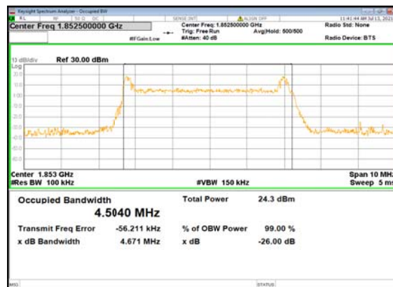
N2(5M)_DFT-s-OFDM_QPSK_Outer_Full_Low_CH
