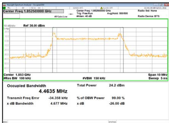
N2(5M)_DFT-s-OFDM_PI_2-BPSK_Outer_Full_Low_CH
