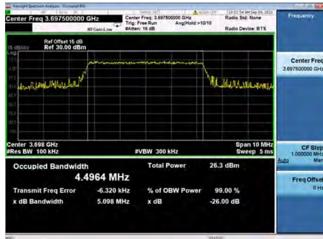
Band48 / 5MHz / High CH / 64QAM
