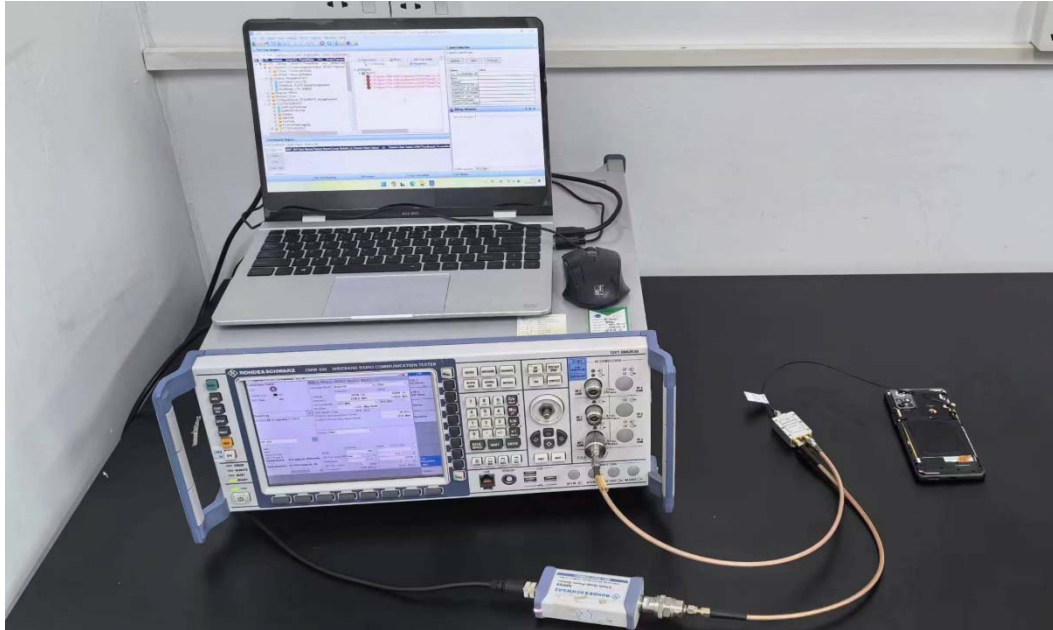
Test setup
