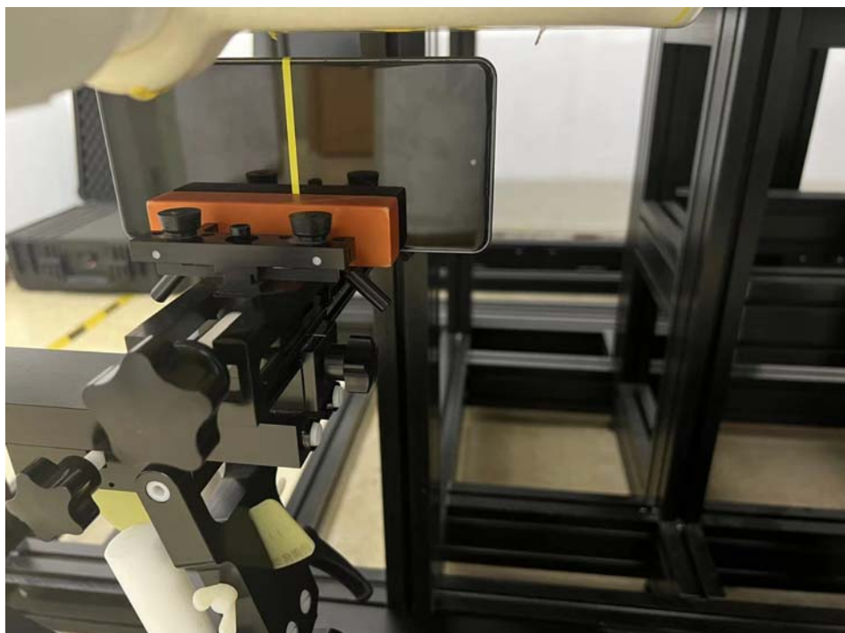
Left side of the SAR measurement
