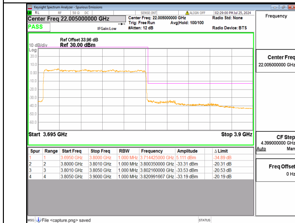
n78(3700-3800MHz) 100M DFT-s-OFDM QPSK Outer_Full High
