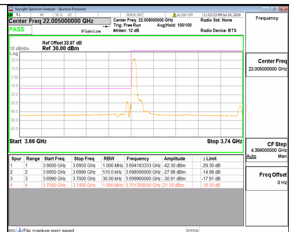
n78(3700-3800MHz) 40M DFT-s-OFDM QPSK Edge_1RB_Left Low
