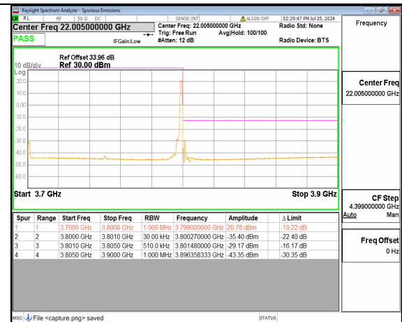
n78(3700-3800MHz) 100M DFT-s-OFDM QPSK Edge_1RB_Right High
