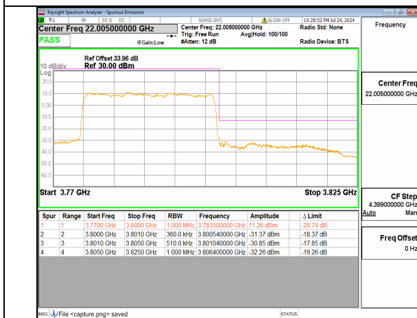
n78(3700-3800MHz) 25M DFT-s-OFDM QPSK Outer_Full High
