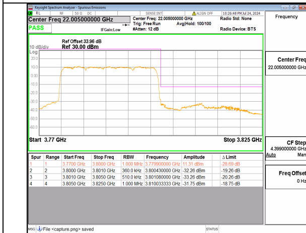
n78(3700-3800MHz) 25M DFT-s-OFDM BPSK Outer_Full High
