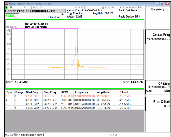
n78(3700-3800MHz) 70M DFT-s-OFDM BPSK Edge_1RB_Right High
