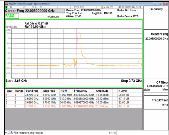
n78(3700-3800MHz) 30M DFT-s-OFDM BPSK Edge_1RB_Left Low
