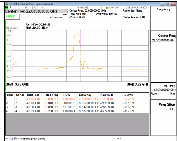
n78(3700-3800MHz) 20M DFT-s-OFDM QPSK Edge_1RB_Right High
