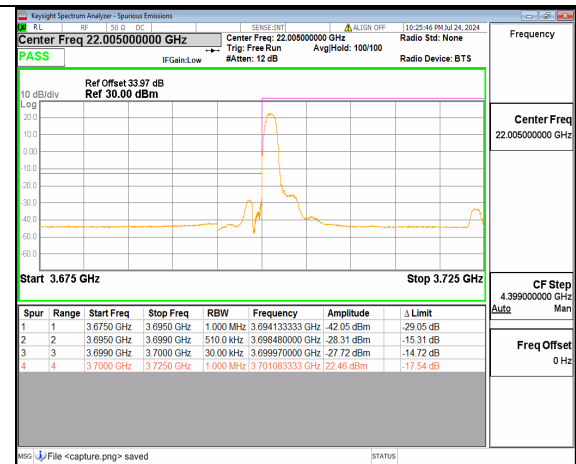
n78(3700-3800MHz) 25M DFT-s-OFDM QPSK Edge_1RB_Left Low
