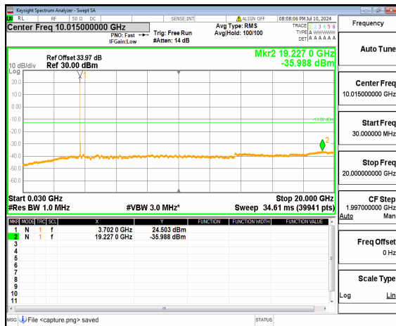
n77(3700-3980MHz) (30MHz-20GHz) 25M DFT-s-OFDM QPSK Inner_1RB_Left Low
