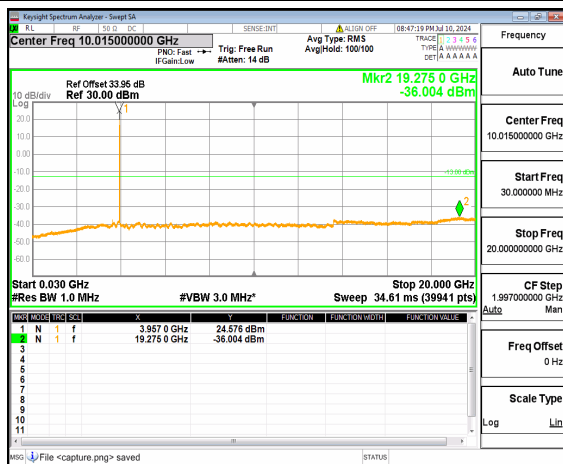
n77(3700-3980MHz) (30MHz-20GHz) 25M DFT-s-OFDM QPSK Inner_1RB_Left High
