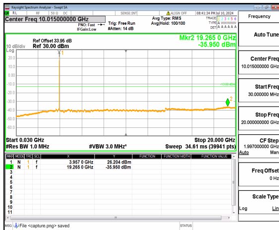
n77(3700-3980MHz) (30MHz-20GHz) 25M DFT-s-OFDM BPSK Inner_1RB_Left High
