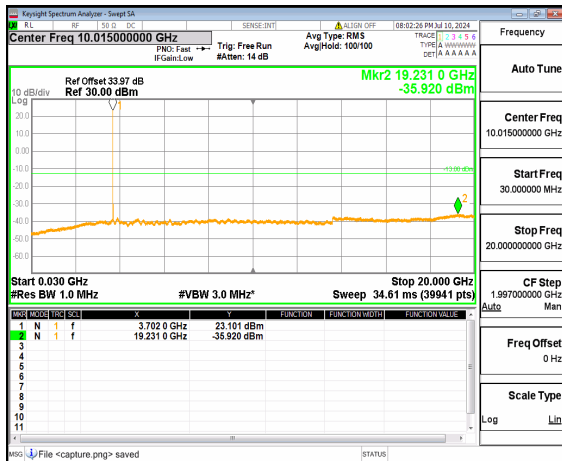
n77(3700-3980MHz) (30MHz-20GHz) 25M DFT-s-OFDM BPSK Inner_1RB_Left Low
