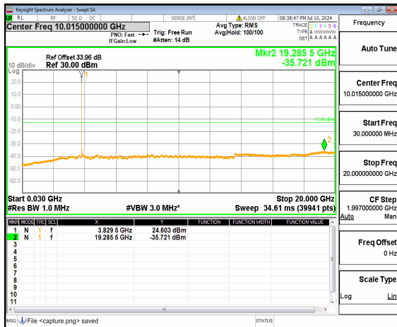
n77(3700-3980MHz) (30MHz-20GHz) 25M DFT-s-OFDM QPSK Inner_1RB_Left Mid
