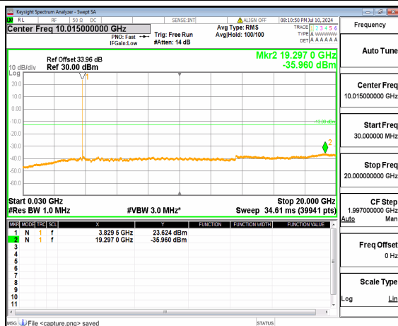
n77(3700-3980MHz) (30MHz-20GHz) 25M DFT-s-OFDM BPSK Inner_1RB_Left Mid
