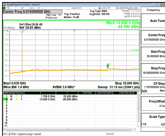
n66 (30MHz-18GHz) 25M DFT-s-OFDM BPSK Inner_1RB_Left High
