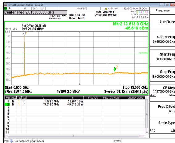
n66 (30MHz-18GHz) 30M DFT-s-OFDM BPSK Inner_1RB_Right High
