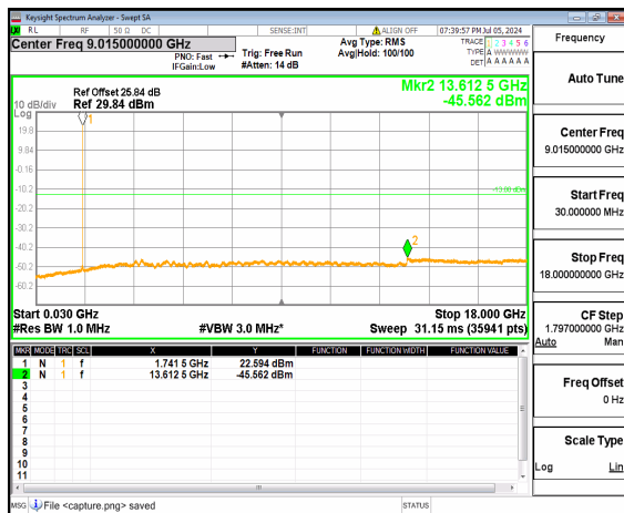
n66 (30MHz-18GHz) 40M DFT-s-OFDM BPSK Inner_1RB_Left High
