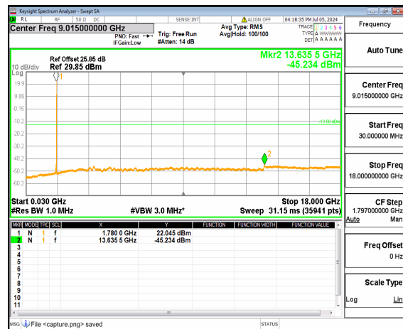
n66 (30MHz-18GHz) 25M DFT-s-OFDM BPSK Inner_1RB_Right High
