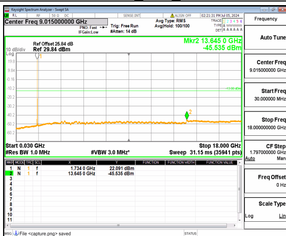
n66 (30MHz-18GHz) 25M DFT-s-OFDM BPSK Inner_1RB_Left Mid
