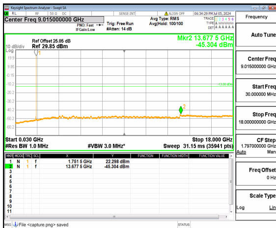
n66 (30MHz-18GHz) 30M DFT-s-OFDM BPSK Inner_1RB_Left High
