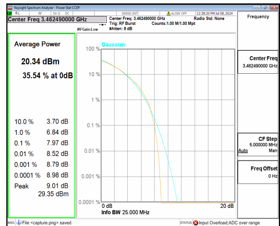
n77(3450-3550MHz) 25M CP-OFDM 256QAM Outer_Full Low
