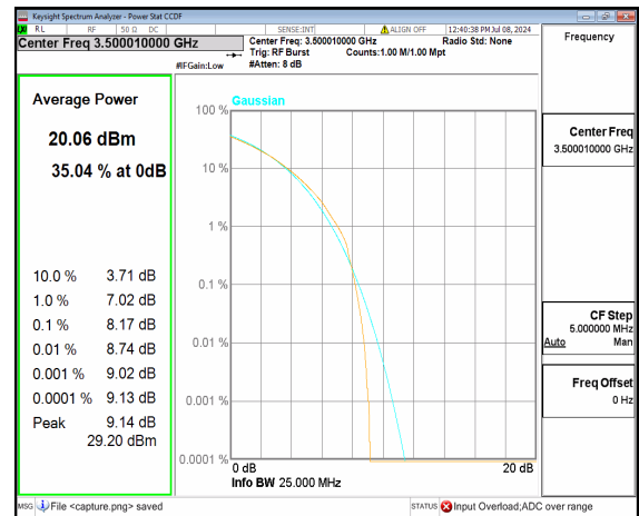
n77(3450-3550MHz) 25M CP-OFDM 256QAM Outer_Full Mid
