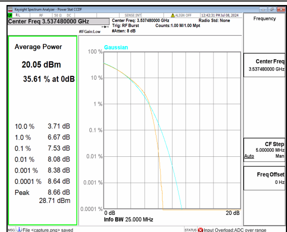
n77(3450-3550MHz) 25M CP-OFDM 256QAM Outer_Full High
