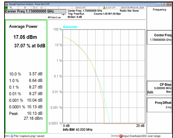
n66 40M CP-OFDM 256QAM Outer_Full Low
