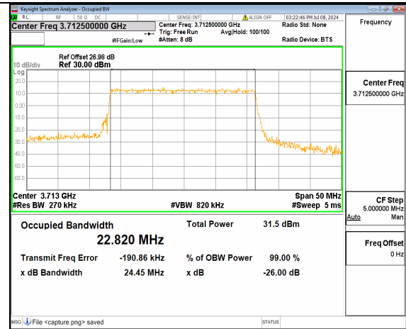
n77(3700-3980MHz) 25M DFT-s-OFDM 64QAM Outer_Full Low
