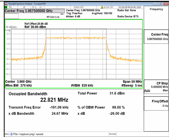
n77(3700-3980MHz) 25M DFT-s-OFDM 64QAM Outer_Full High
