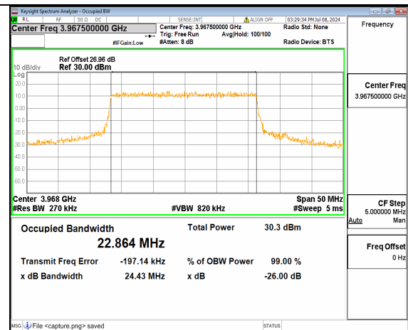
n77(3700-3980MHz) 25M CP-OFDM QPSK Outer_Full High
