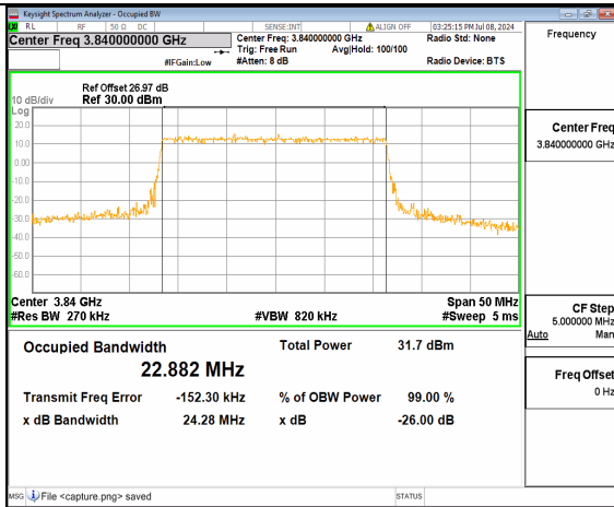
n77(3700-3980MHz) 25M DFT-s-OFDM 16QAM Outer_Full Mid
