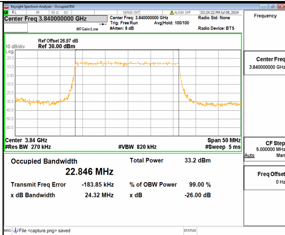
n77(3700-3980MHz) 25M DFT-s-OFDM BPSK Outer_Full Mid
