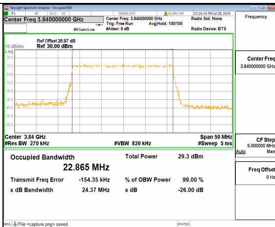
n77(3700-3980MHz) 25M DFT-s-OFDM 256QAM Outer_Full Mid
