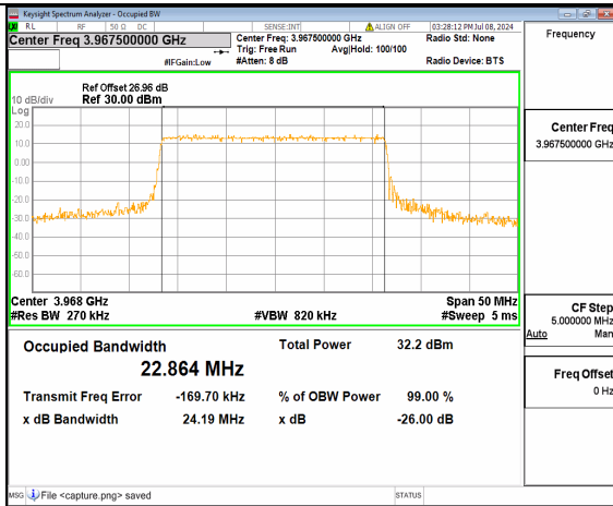
n77(3700-3980MHz) 25M DFT-s-OFDM 16QAM Outer_Full High
