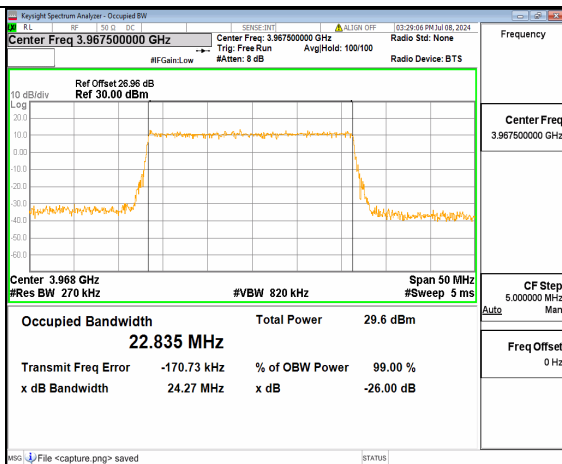
n77(3700-3980MHz) 25M DFT-s-OFDM 256QAM Outer_Full High
