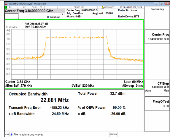
n77(3700-3980MHz) 25M DFT-s-OFDM QPSK Outer_Full Mid
