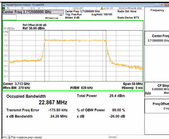
n77(3700-3980MHz) 25M DFT-s-OFDM 256QAM Outer_Full Low
