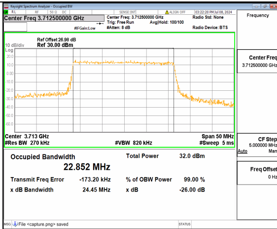
n77(3700-3980MHz) 25M DFT-s-OFDM 16QAM Outer_Full Low
