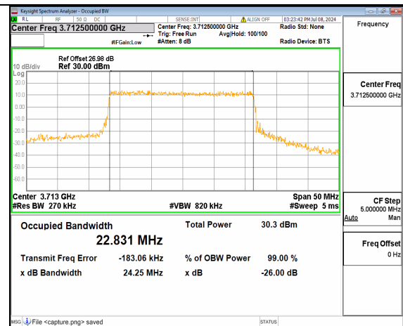
n77(3700-3980MHz) 25M CP-OFDM QPSK Outer_Full Low
