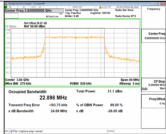
n77(3700-3980MHz) 25M DFT-s-OFDM 64QAM Outer_Full Mid
