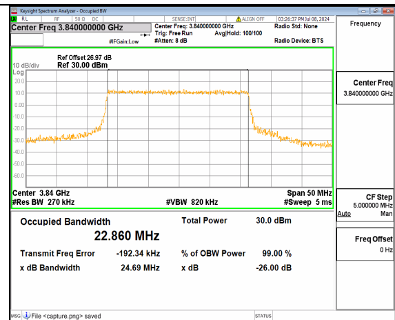
n77(3700-3980MHz) 25M CP-OFDM QPSK Outer_Full Mid
