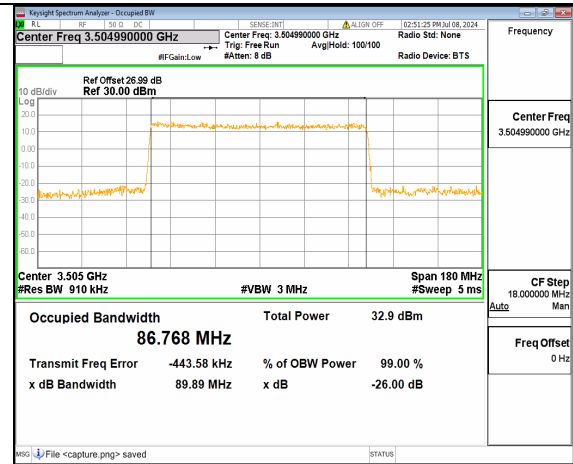
n77(3450-3550MHz) 90M DFT-s-OFDM 64QAM Outer_Full High
