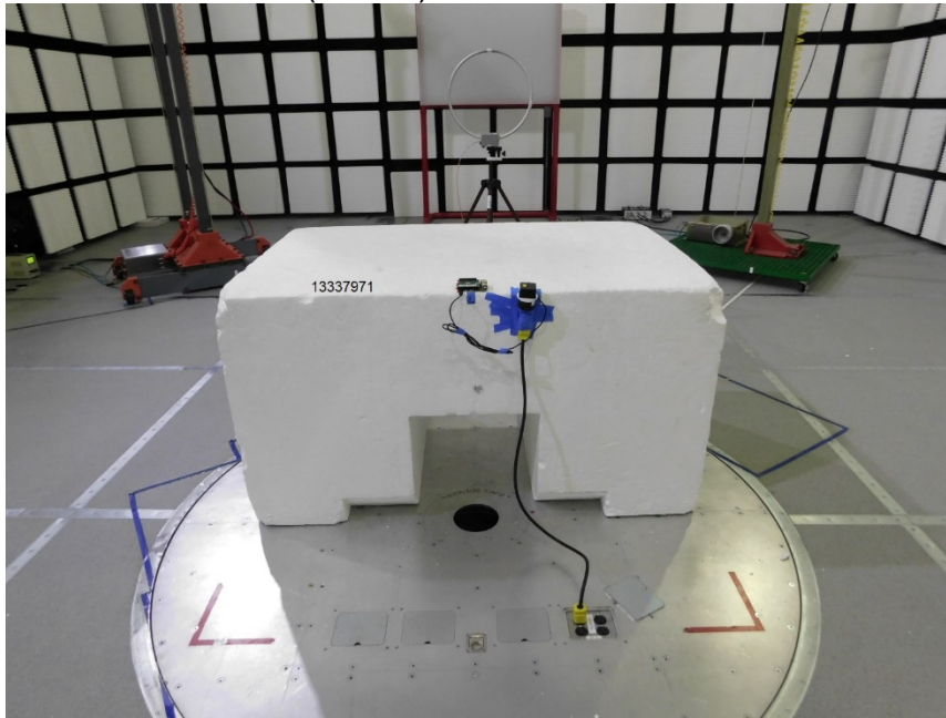
RADIATED PHOTO (<1GHz) 5GHz MODE
