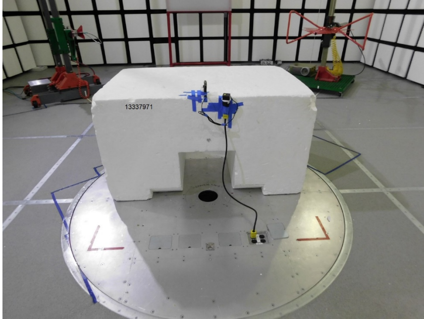
RADIATED PHOTO (<1GHz) 2.4GHz MODE
