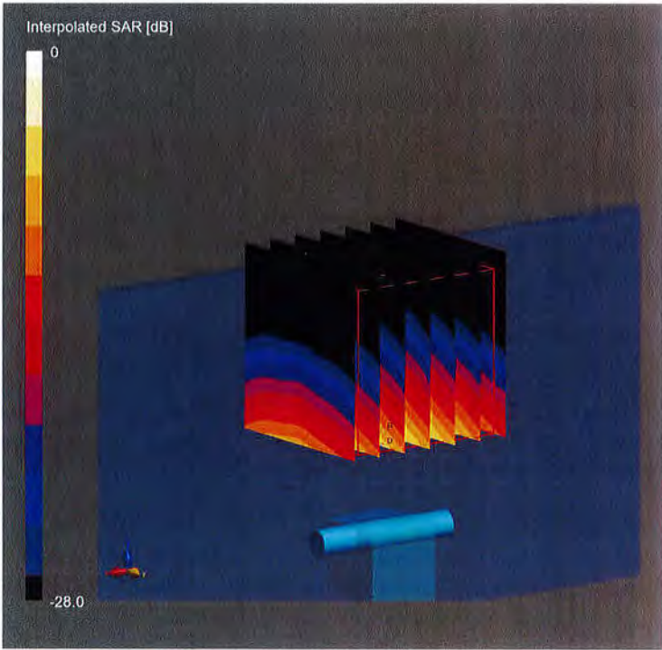
0 dB = 34.7 W/Kg
