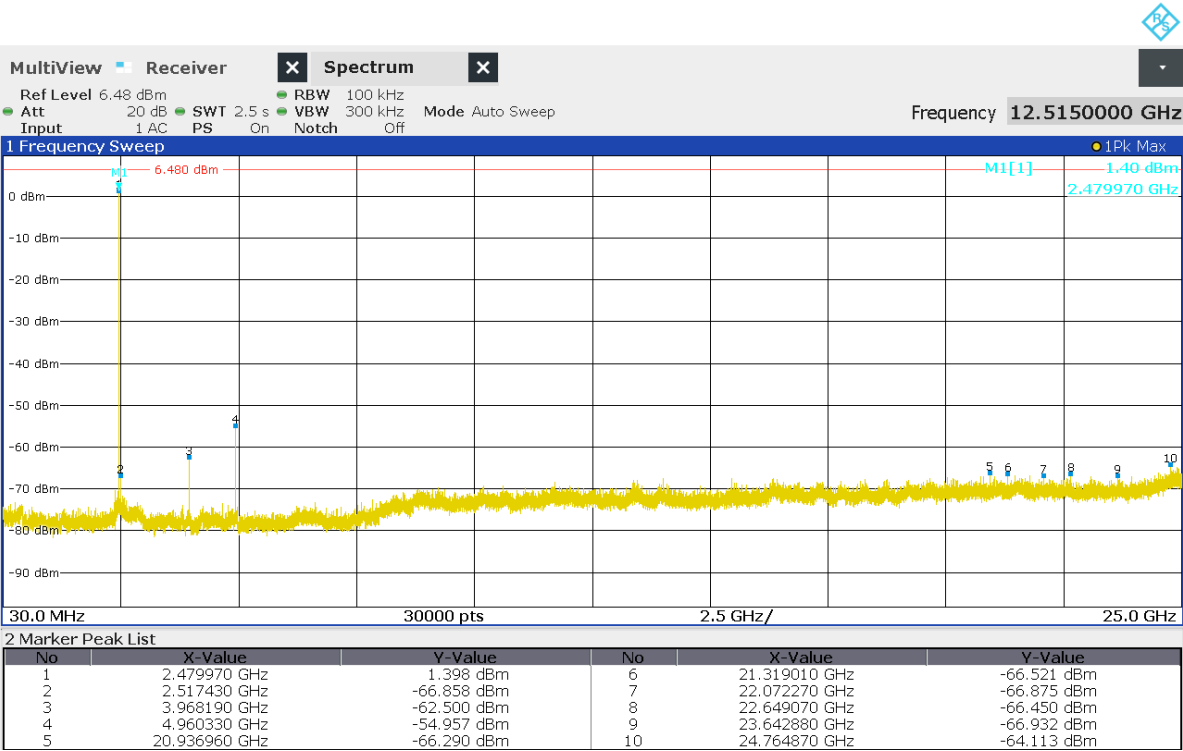
Figure 13 Conducted emissions 30MHz to 25GHz. Operation on channel 2480MHz.
