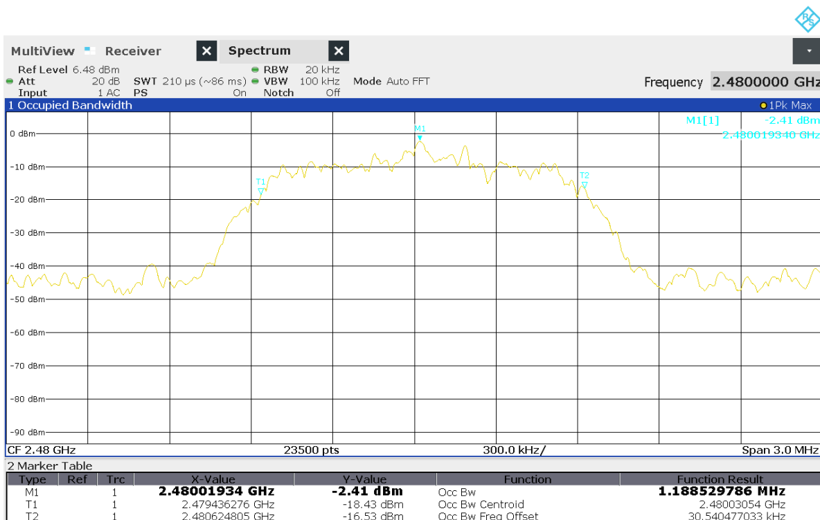
Figure 19 99% Occupied Bandwidth. Operation on channel 2480MHz
