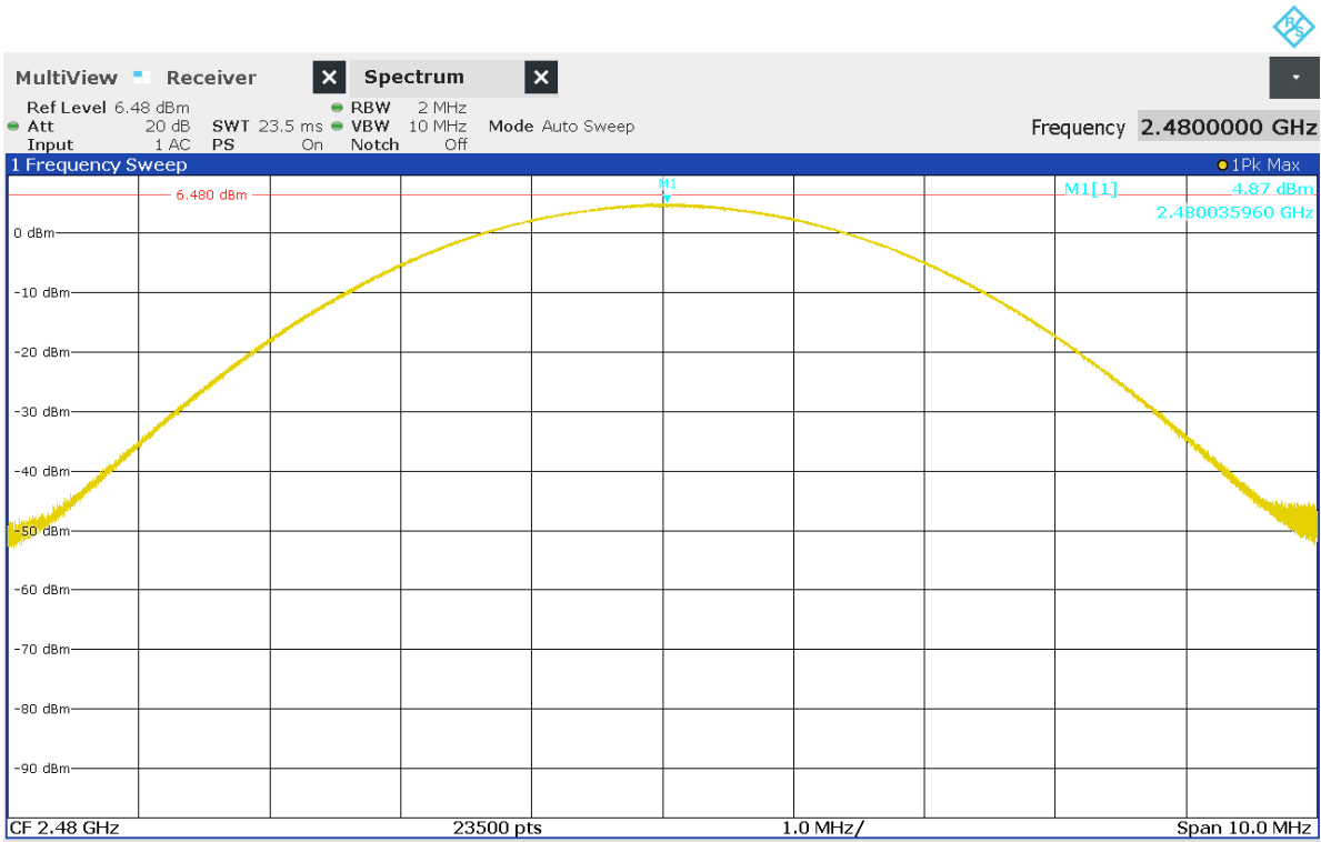
Figure 22 Peak output power, Operation on channel 2480MHz
