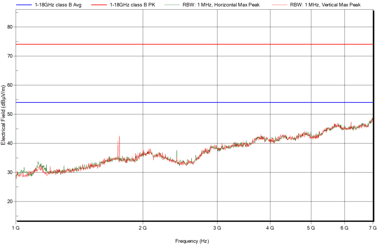
Figure 6 Electric field emissions Plot, 1GHz to 7GHz, Operation on 2402MHz - Peak detector scan
