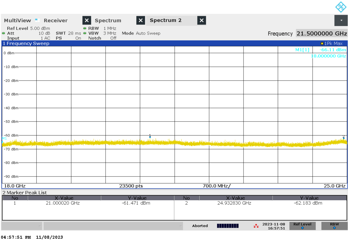
Figure 9 – Manual investigation – Operating on BLE channel 2440MHz
