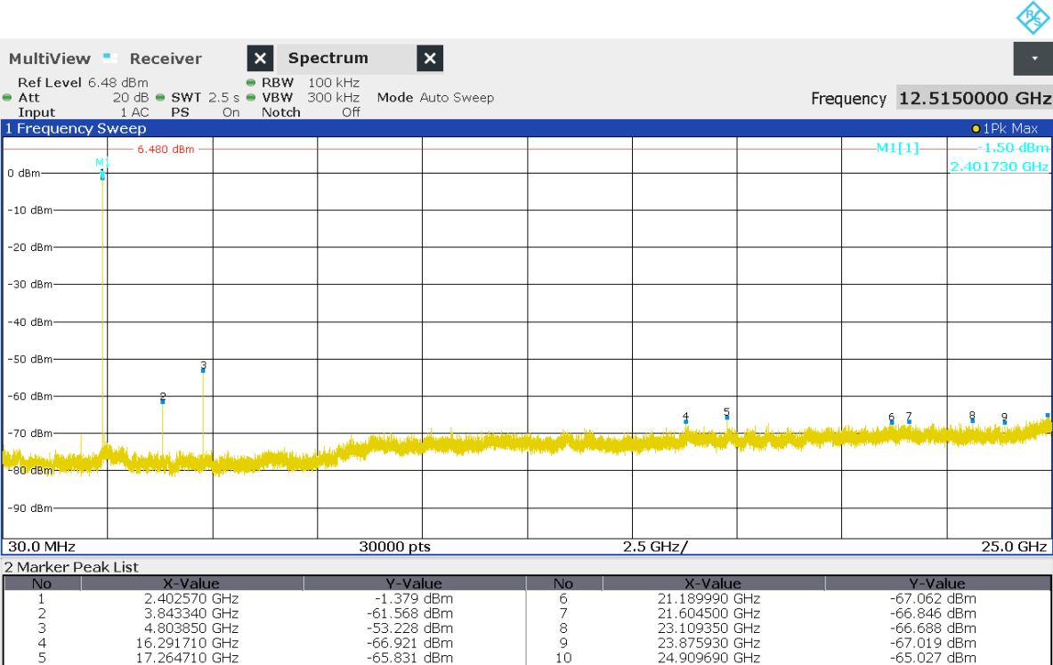
Figure 11 Conducted emissions 30MHz to 25GHz. Operation on channel 2402MHz.
