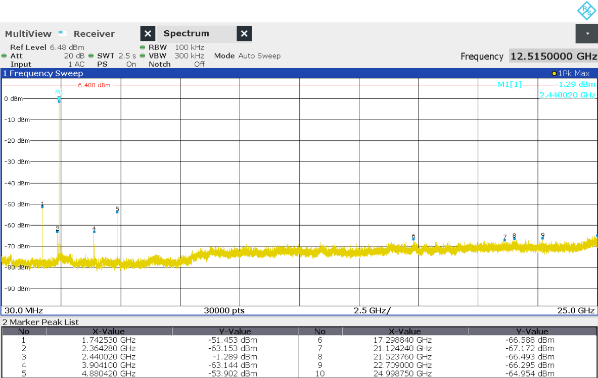
Figure 12 Conducted emissions 30MHz to 25GHz. Operation on channel 2440MHz.
