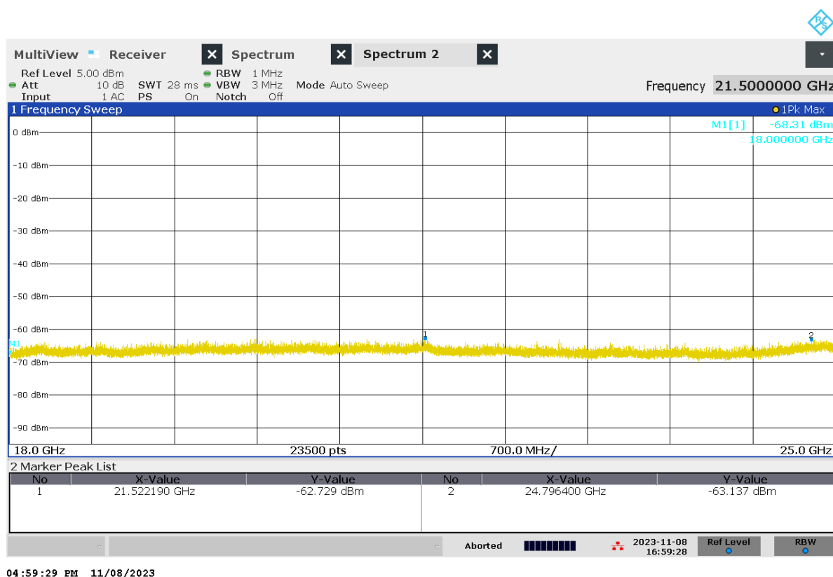
Figure 8 – Manual investigation – Operating on BLE channel 2402MHz
