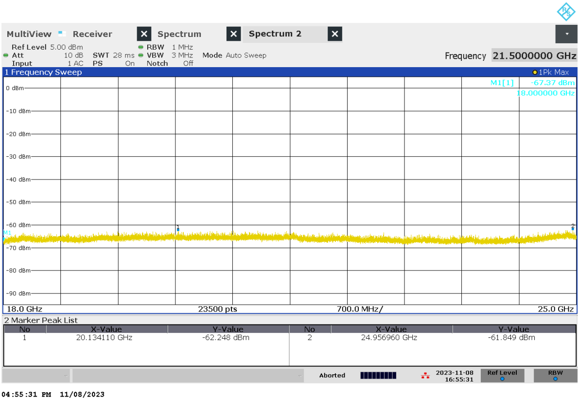
Figure 10 – Manual investigation – Operating on BLE channel 2480MHz
