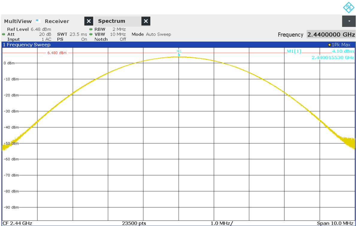
Figure 21 Peak output power, Operation on channel 2440MHz
