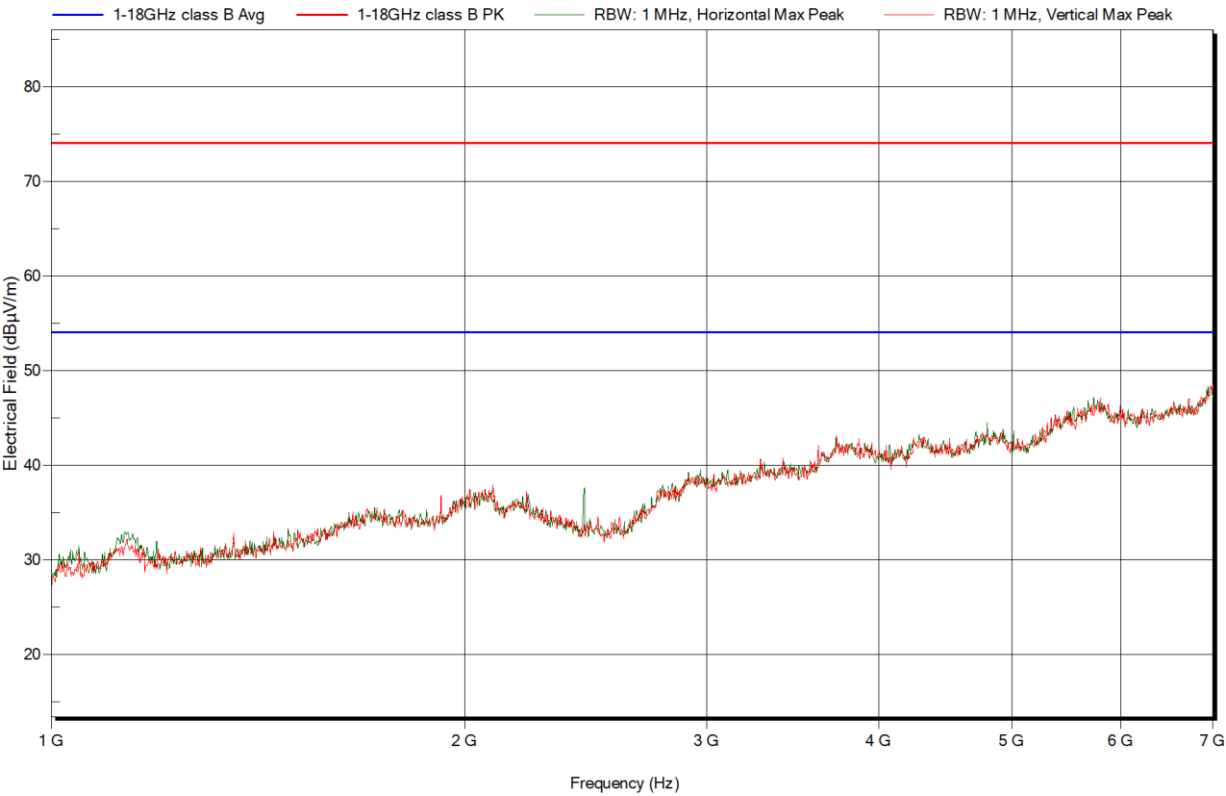
Figure 7 Electric field emissions Plot, 1GHz to 7GHz, Operation on 2440MHz – Peak detector scan
