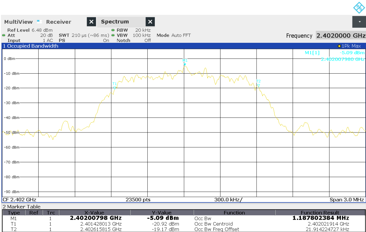
Figure 17 99% Occupied Bandwidth. Operation on channel 2402MHz
