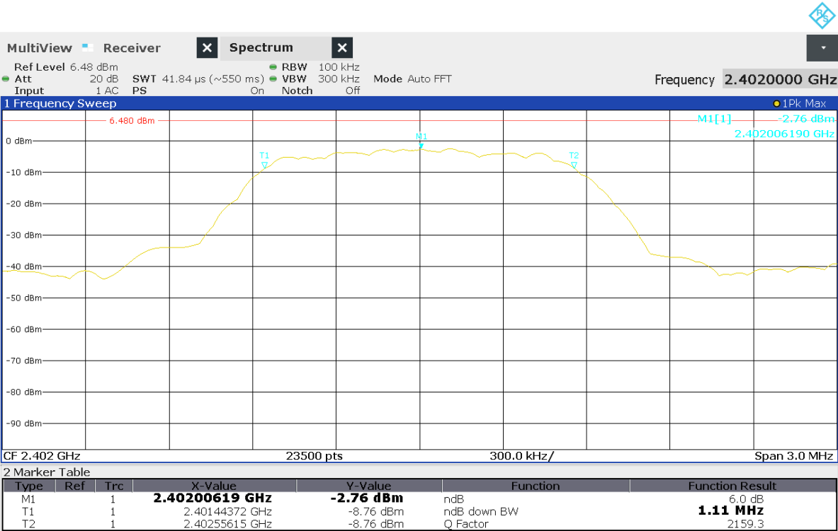
Figure 14 Bandwidth at 6dB Point. Operation on channel 2402MHz
