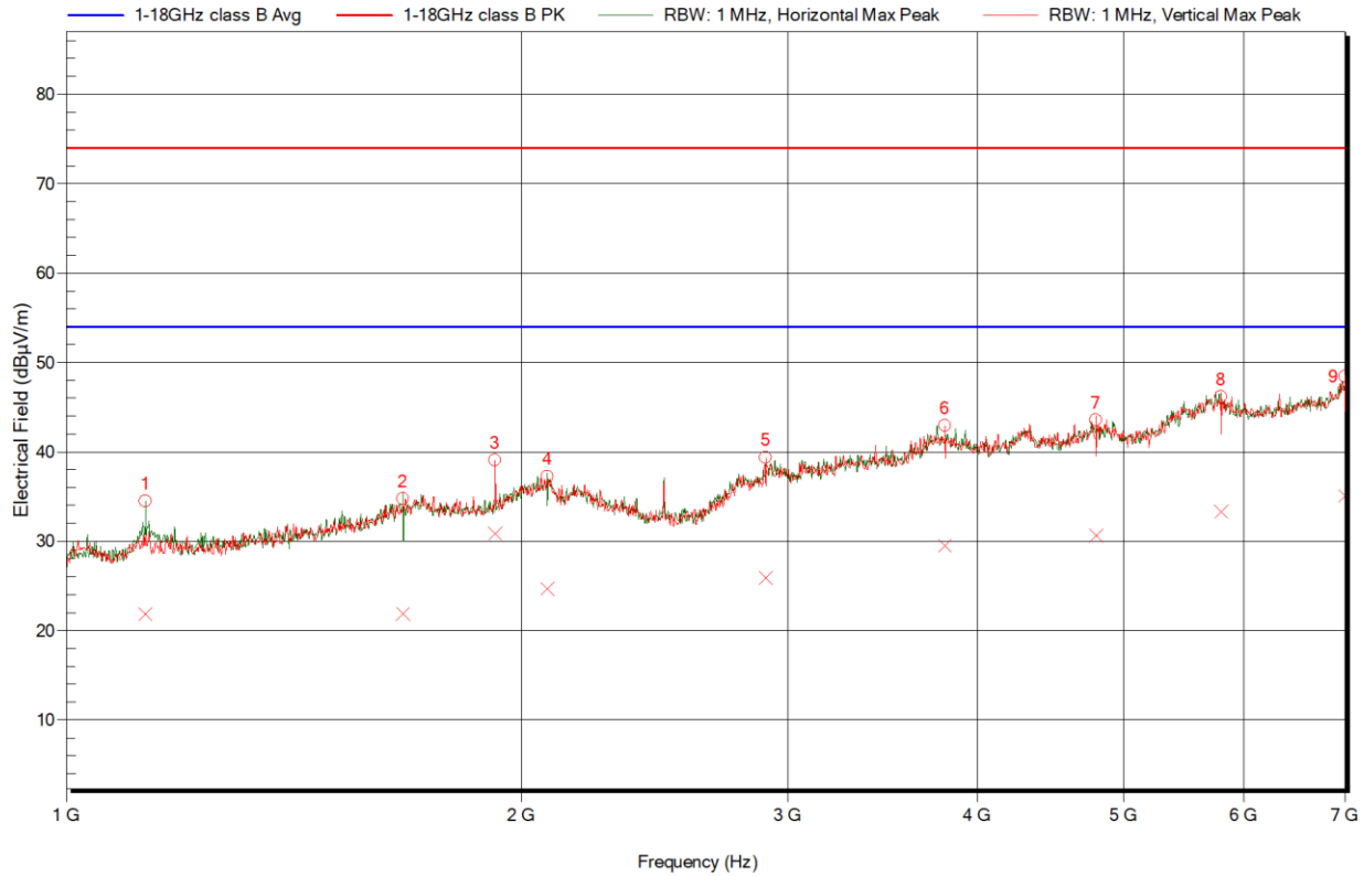
Figure 5 Electric field emissions Plot, 1GHz to 7GHz. Operation on 2480MHz
