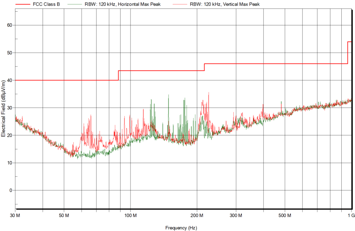
Figure 3 Electric field emissions Plot, 30MHz to 1GHz, Operation on 2402MHz - Peak detector scan
