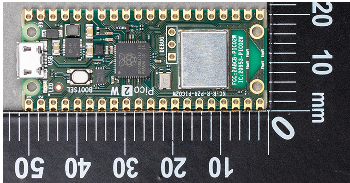
Raspberry Pi Pico 2 W Top
