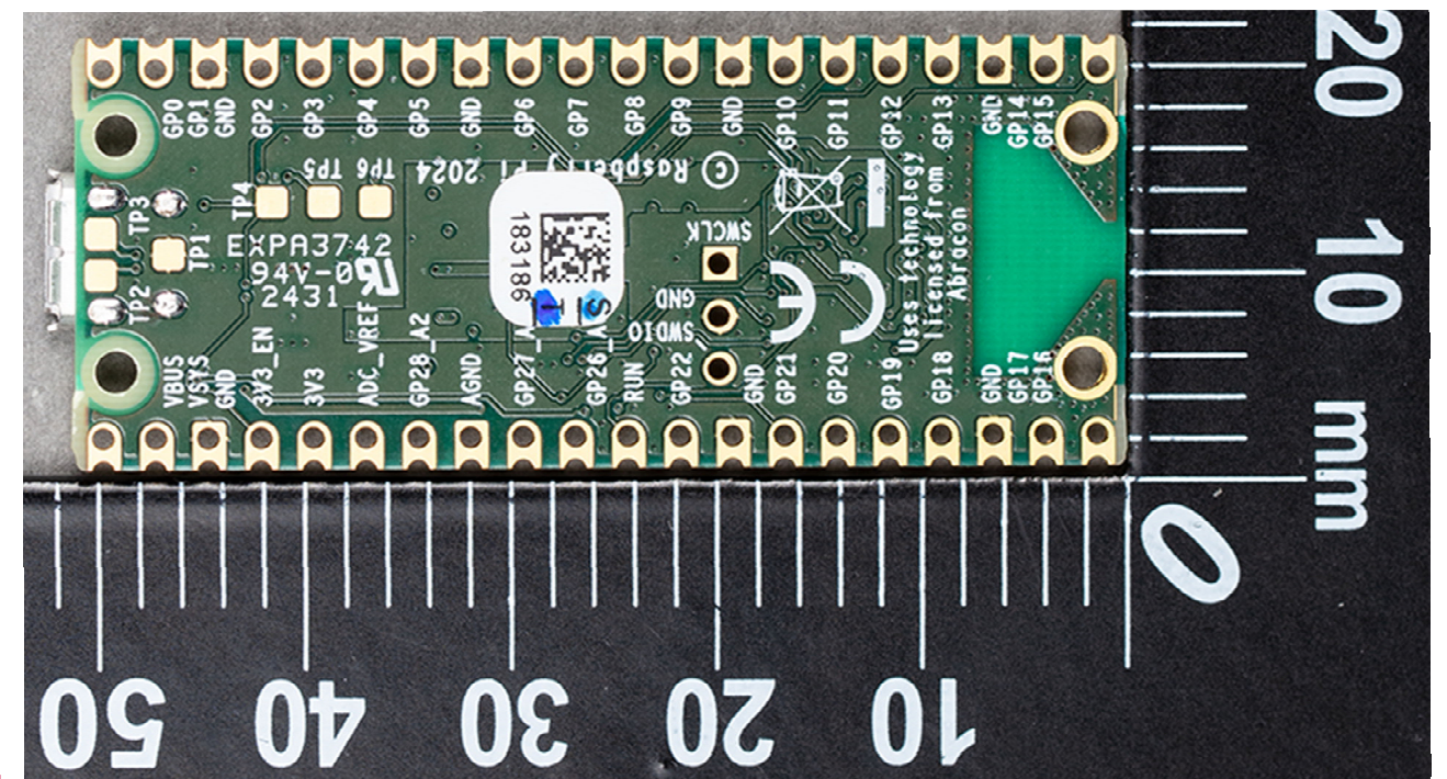
Raspberry Pi Pico 2 W Bottom
