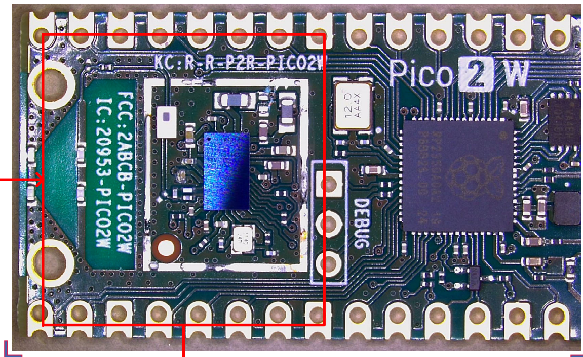
Raspberry Pi Pico 2 W Radio Circuitry without Can
