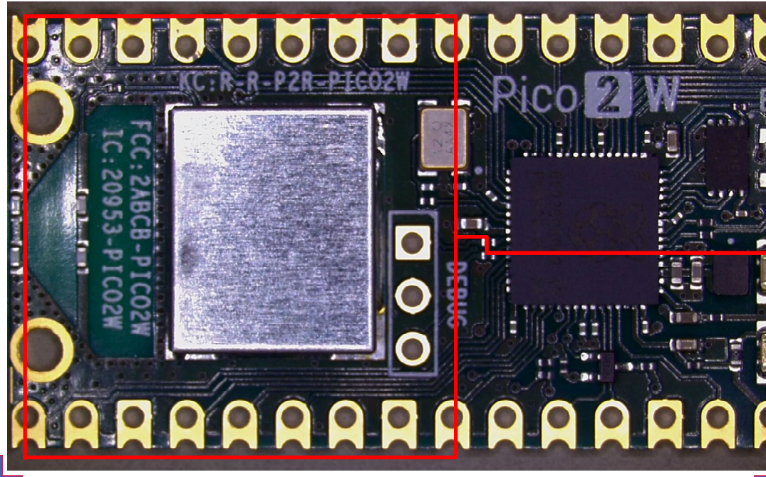
Raspberry Pi Pico 2 W Radio Circuitry with Can
