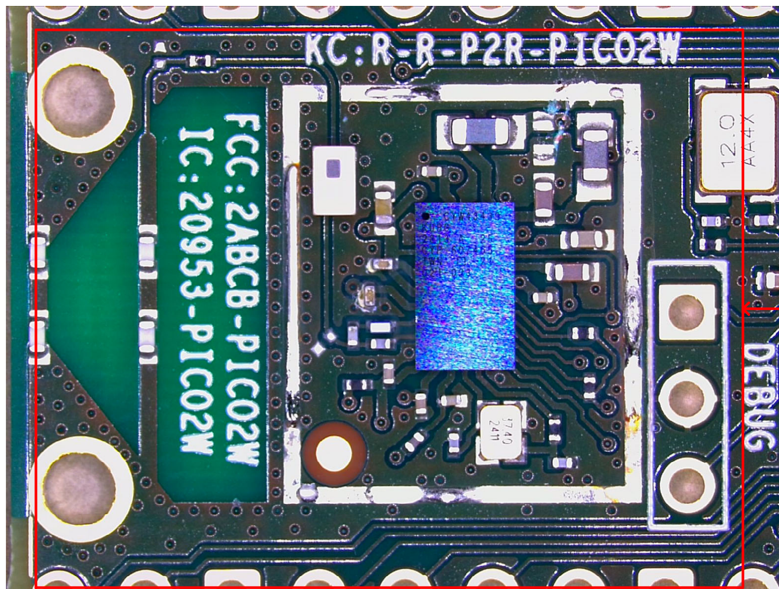
Raspberry Pi Pico 2 W Radio Circuitry without Can Detailed
