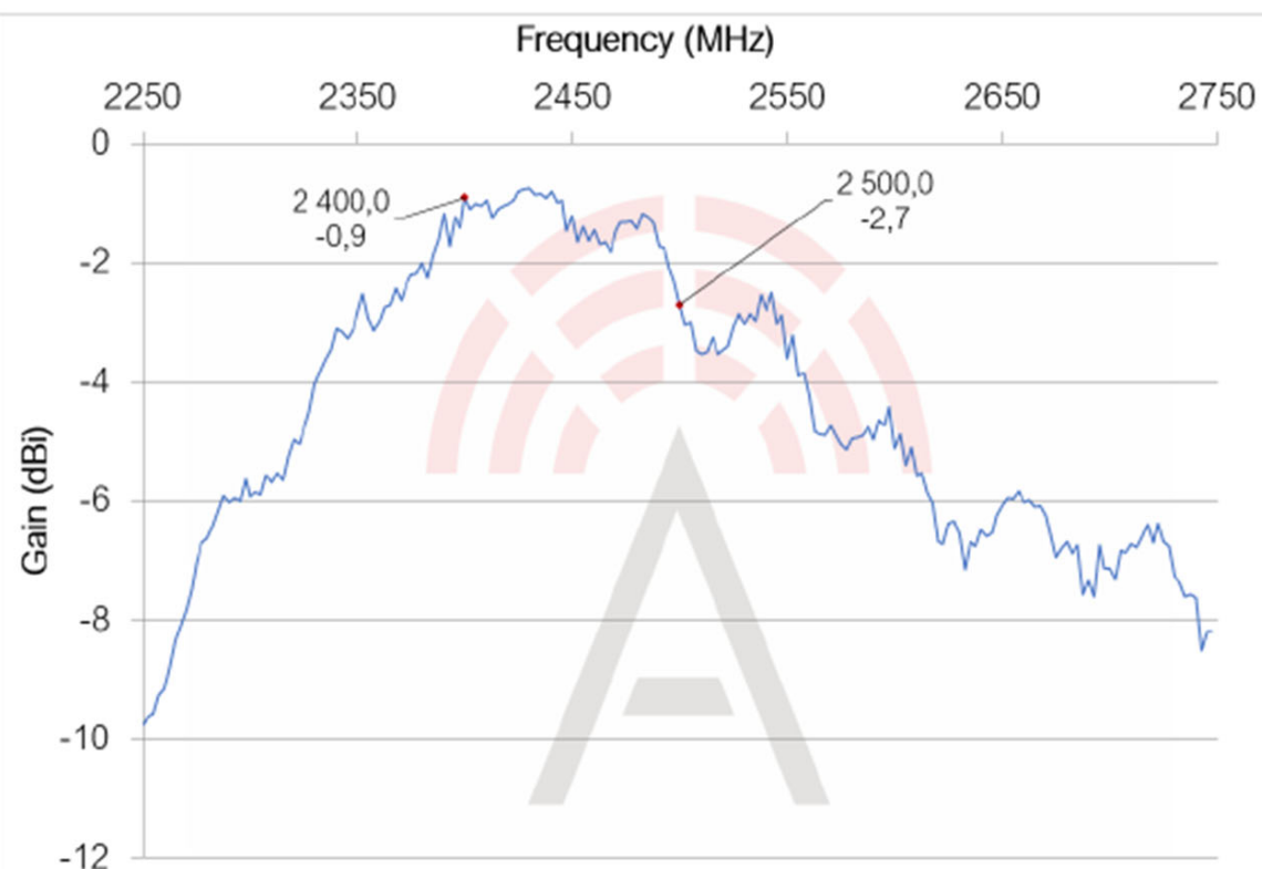
Antenna Gain Plot
