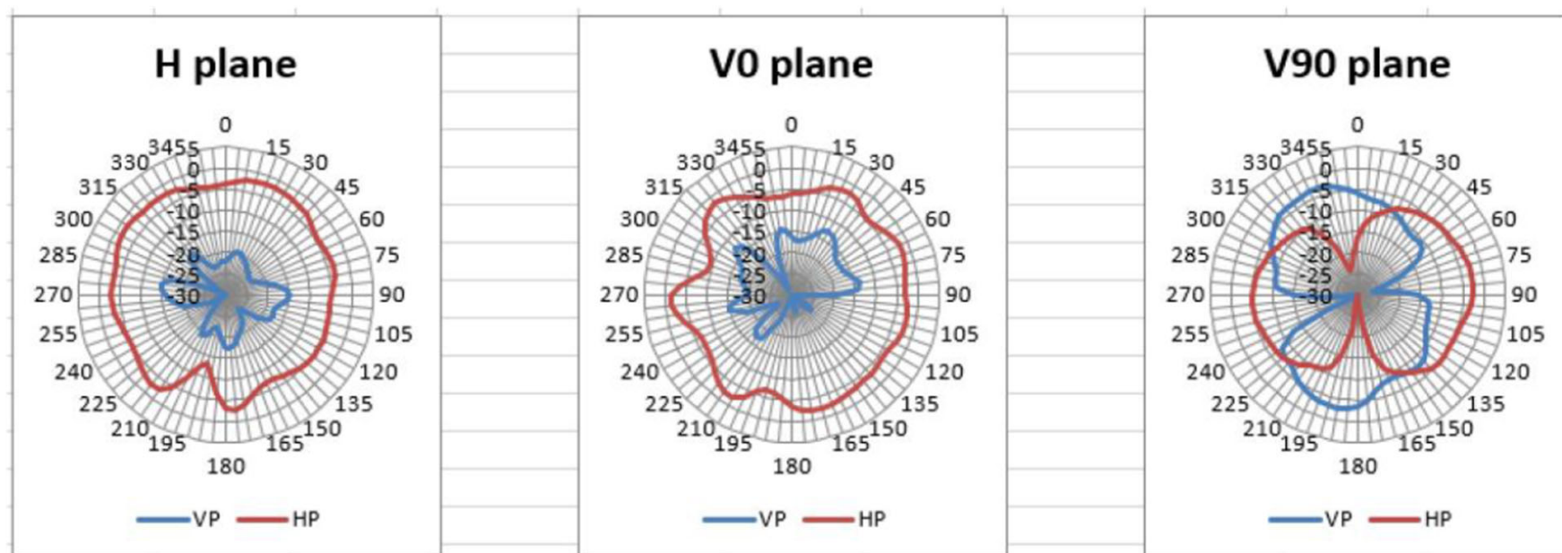
Antenna Radiation Pattern – 3 Axis
