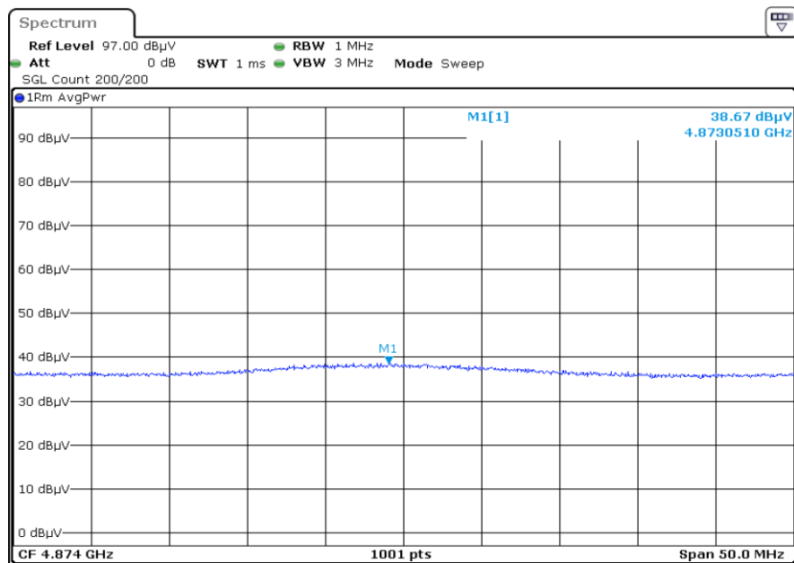
F2 X2 4874.0 Harmonic Vertical AVG
