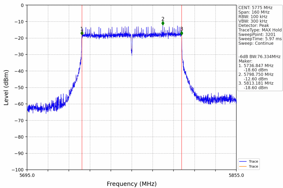
802.11ac(VHT80)_MCH_5775MHz_Ant1_NTNV
