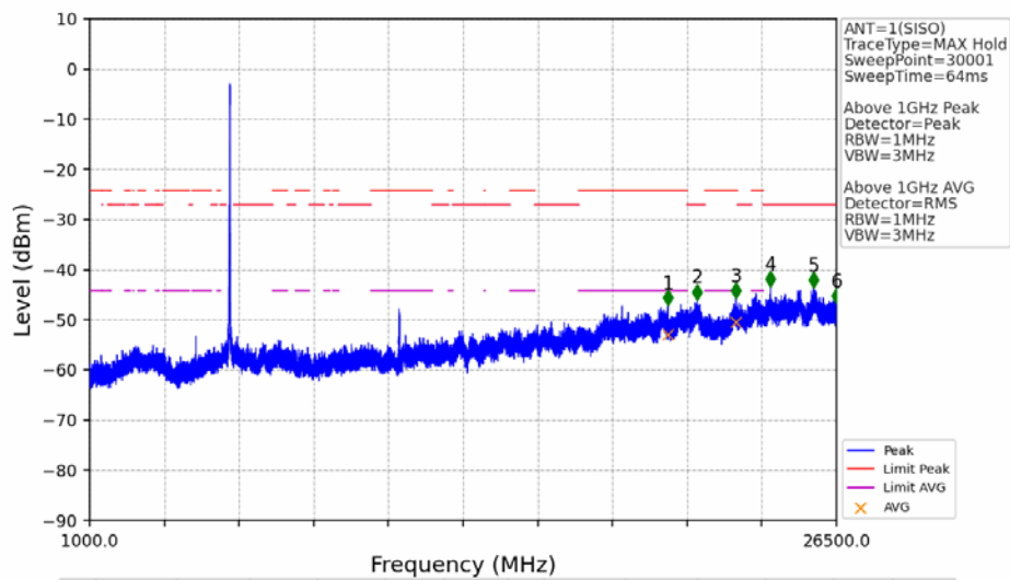
802.11ax(HEW20)_MCH_5785MHz_RU242_Left_Ant1_NTNV
