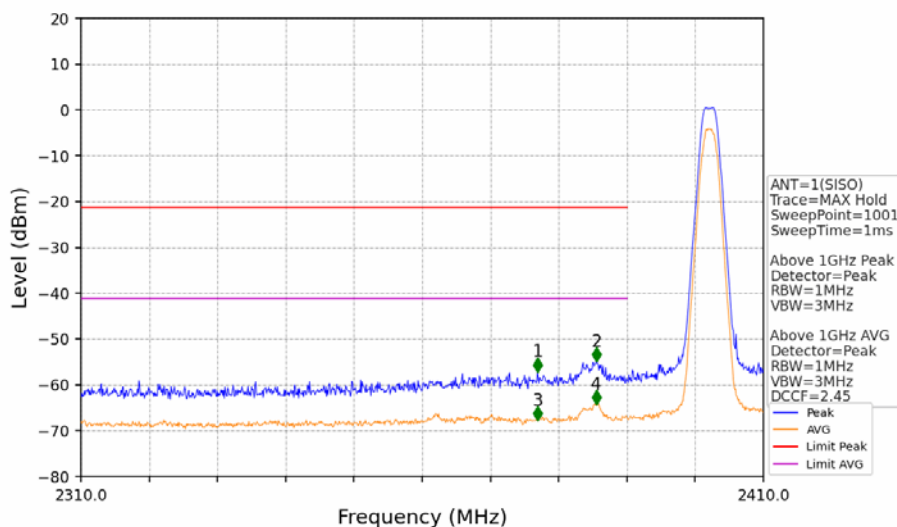
2M_LCH_2402MHz_Ant1_NTNV
