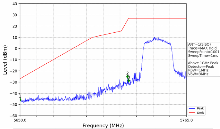
802.11ax(HEW20)_LCH_5745MHz_RU242_Left_Ant1_NTNV
