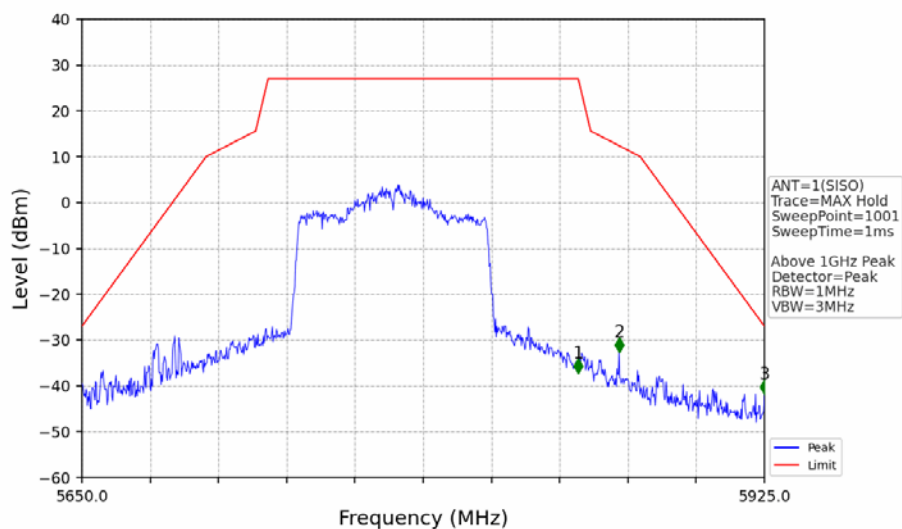
802.11ac(VHT80)_MCH_5775MHz_Ant1_NTNV
