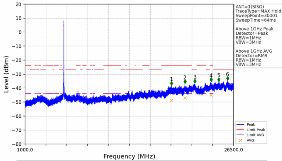
802.11ax(HEW20)_LCH_5745MHz_RU242_Left_Ant1_NTNV
