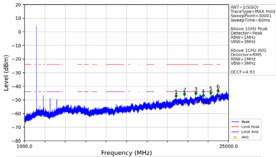
2M_LCH_2402MHz_Ant1_NTNV
