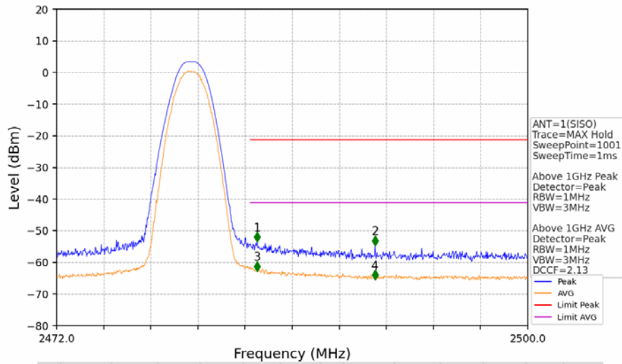
1M_HCH_2480MHz_Ant1_NTNV
