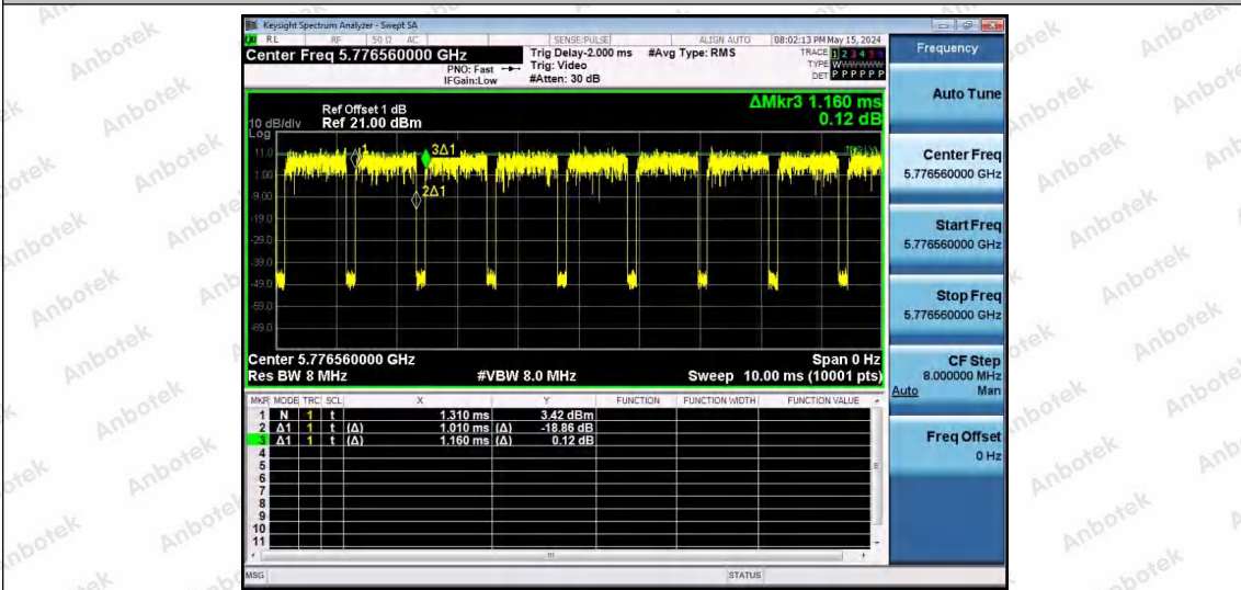
NTNV-11AX40SISO-Ant1-5795-26Tone-RU0
