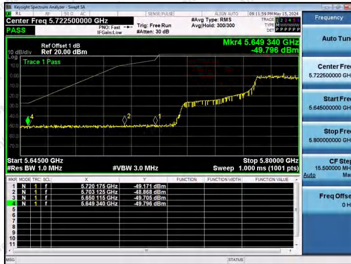
11AX80SISO-Ant1-5775-484Tone-RU66-PASS
