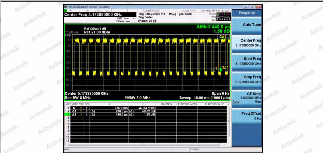
NTNV-11AX80SISO-Ant1-5210-106Tone-RU53
