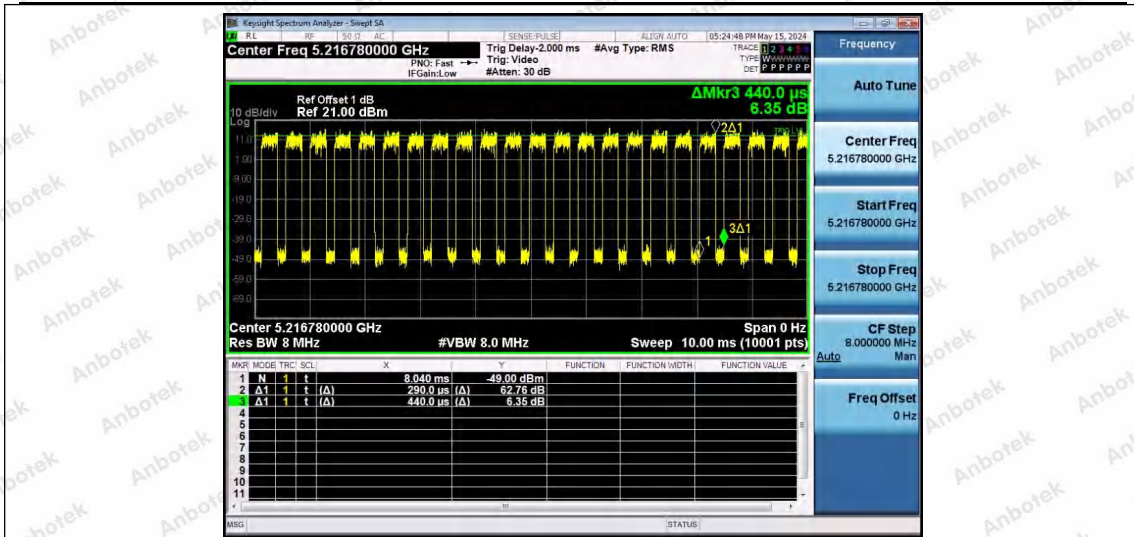
NTNV-11AX40SISO-Ant1-5230-106Tone-RU53
