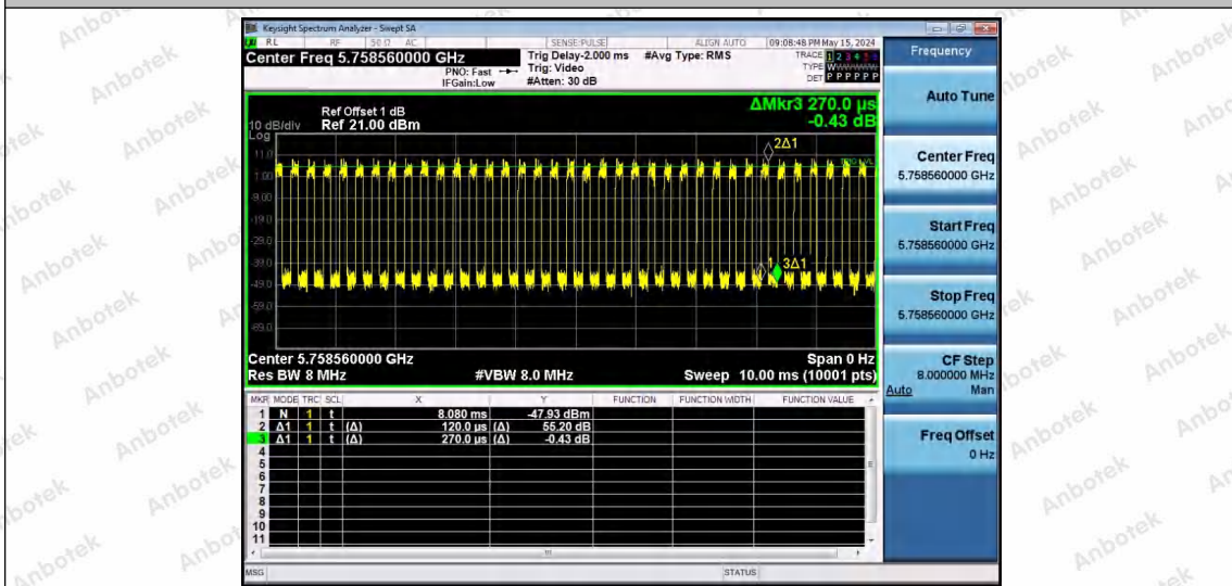
NTNV-11AX80SISO-Ant1-5775-484Tone-RU65
