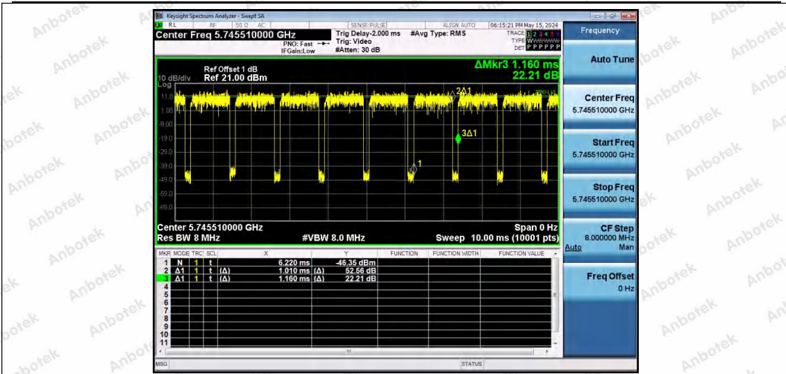
NTNV-11AX20SISO-Ant1-5745-26Tone-RU4
