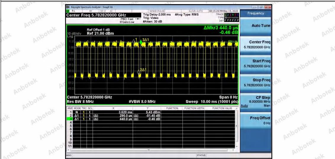
NTNV-11AX40SISO-Ant1-5795-106Tone-RU53
