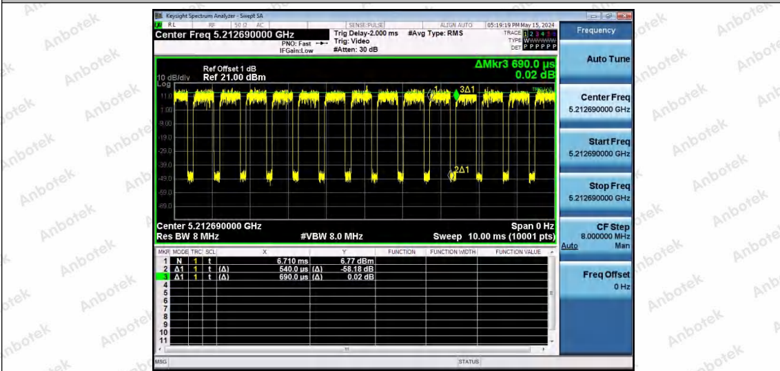
NTNV-11AX40SISO-Ant1-5230-52Tone-RU37
