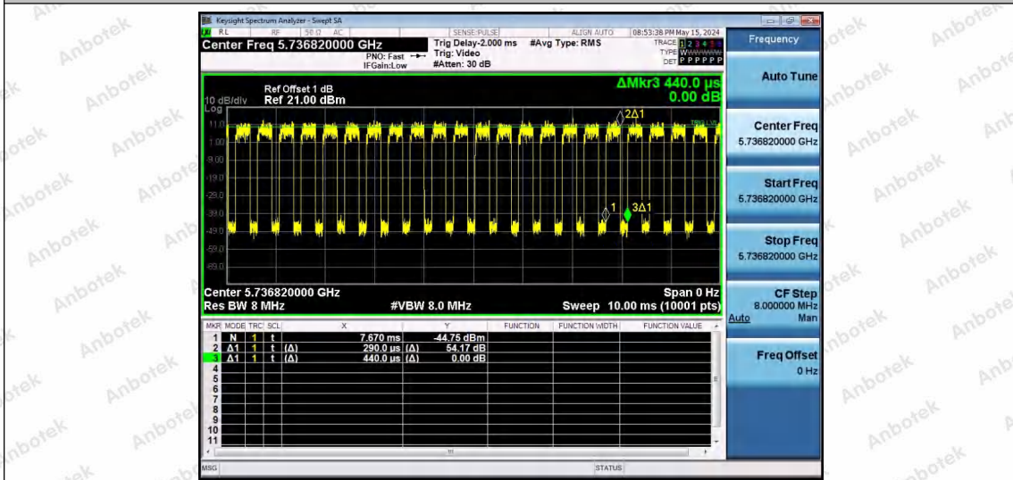
NTNV-11AX80SISO-Ant1-5775-106Tone-RU53
