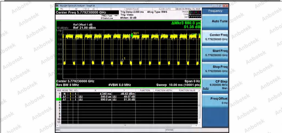
NTNV-11AX40SISO-Ant1-5795-52Tone-RU37
