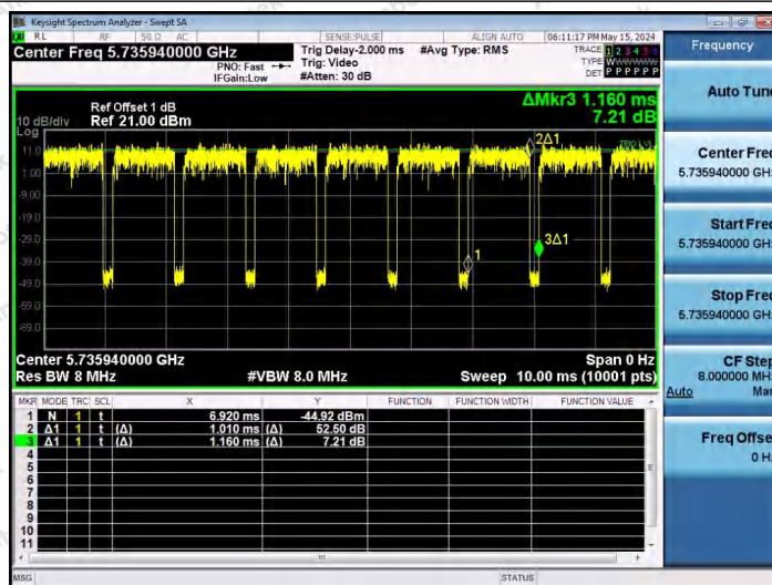
NTNV-11AX20SISO-Ant1-5745-26Tone-RU0
