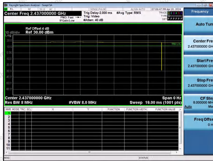
NTNV-11B-Ant2-2437
