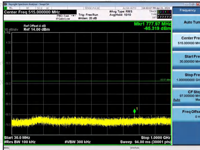
11AX20MIMO-Ant2-2437-30~1000-PASS
