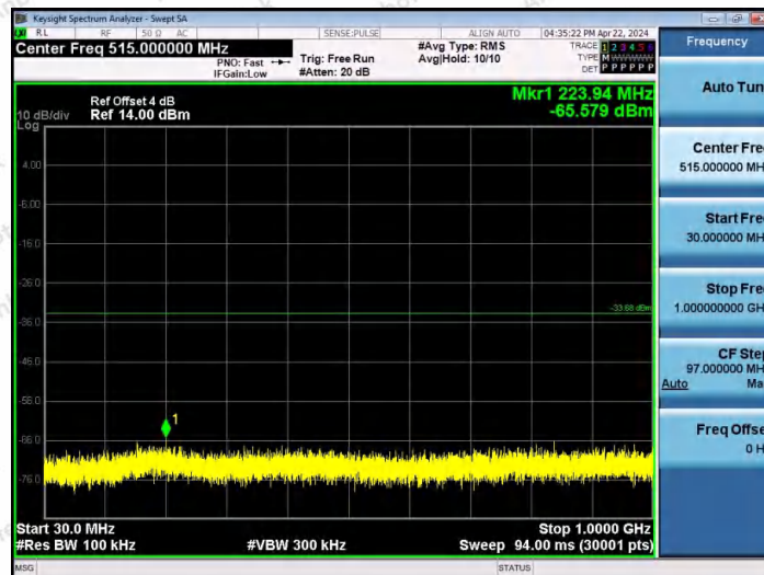
11AX20MIMO-Ant1-2412-30~1000-PASS
