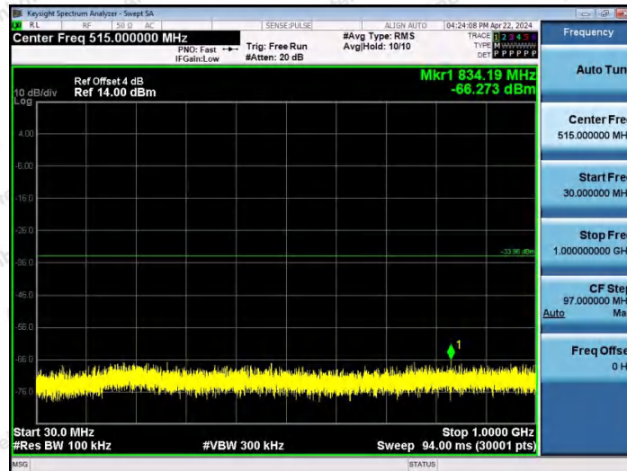
11N20MIMO-Ant2-2412-30~1000-PASS
