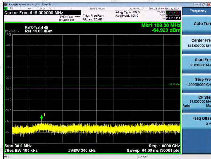
11G-Ant2-2412-30~1000-PASS
