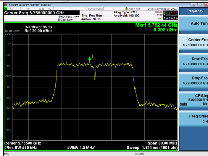
11AC40SISO_Ant2_5755
