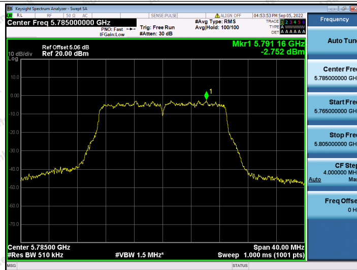
11AC20SISO_Ant2_5785
