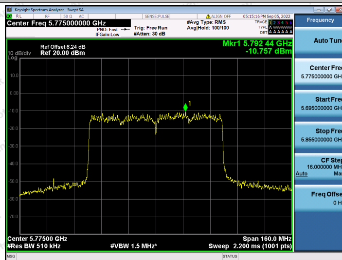
11AX80SISO_Ant2_5775
