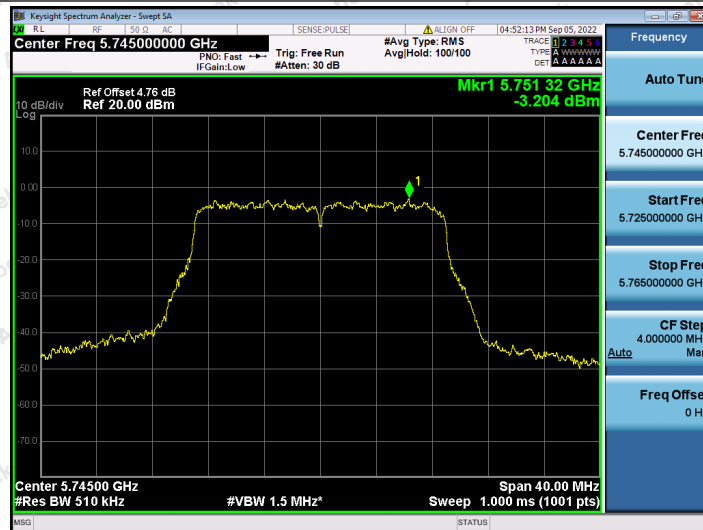
11AC20SISO_Ant2_5745
