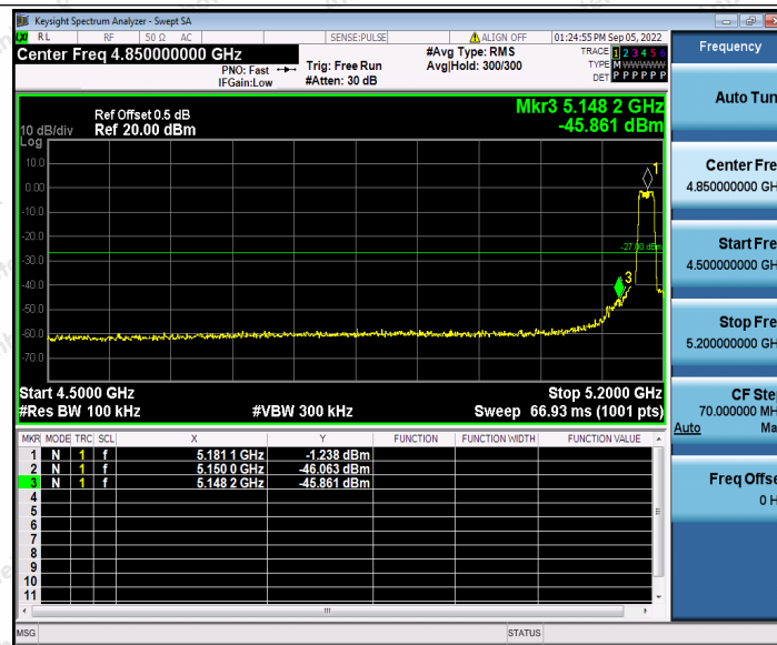
11AC20SISO_Ant2_Low_5180
