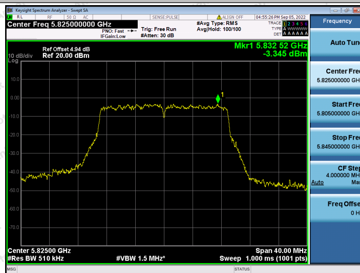
11AC20SISO_Ant2_5825
