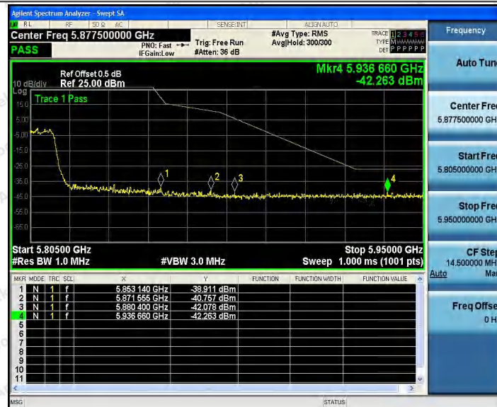
11AX80SISO_Ant2_Low_5775
