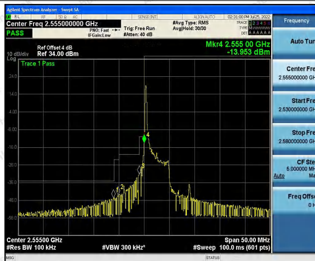
Band41-5MHz-QPSK-40265-1RB#24
