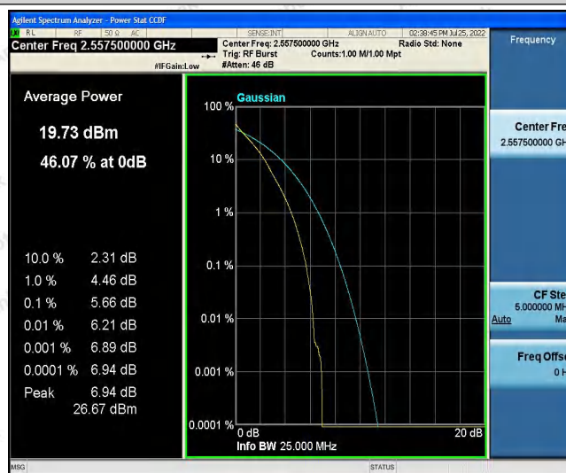
Band41-5MHz-QPSK-40690-1RB#0
