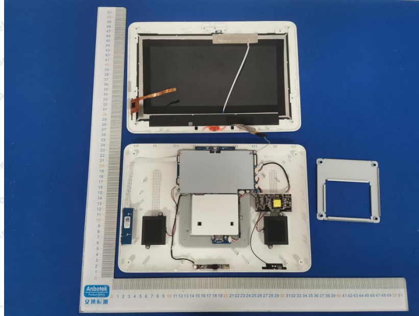
WIFI Antenna
