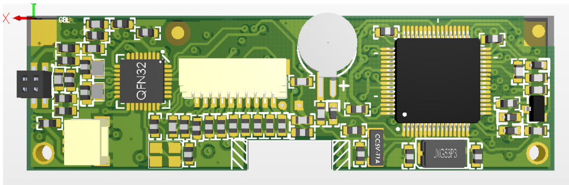
Figure 2: PCB bottom side
