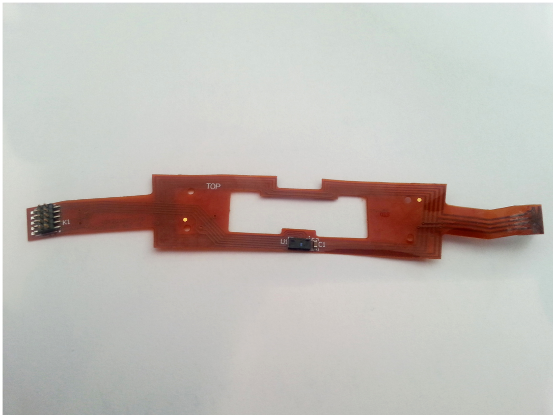
Figure 1: Top layout
