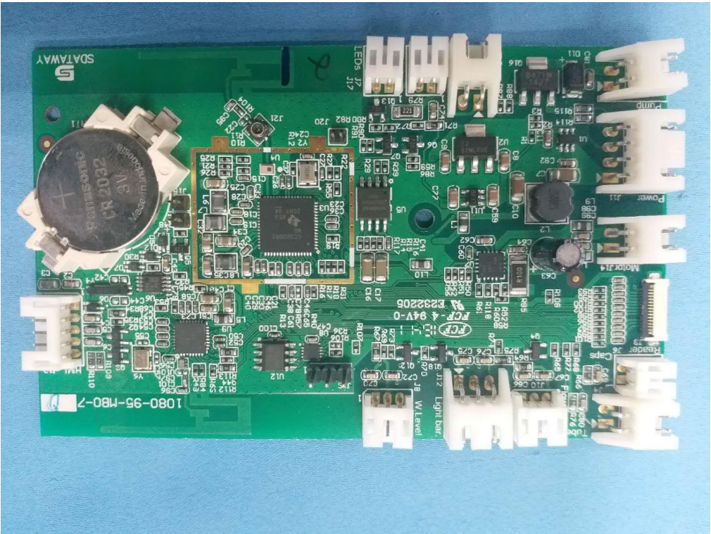
Wireless module board
