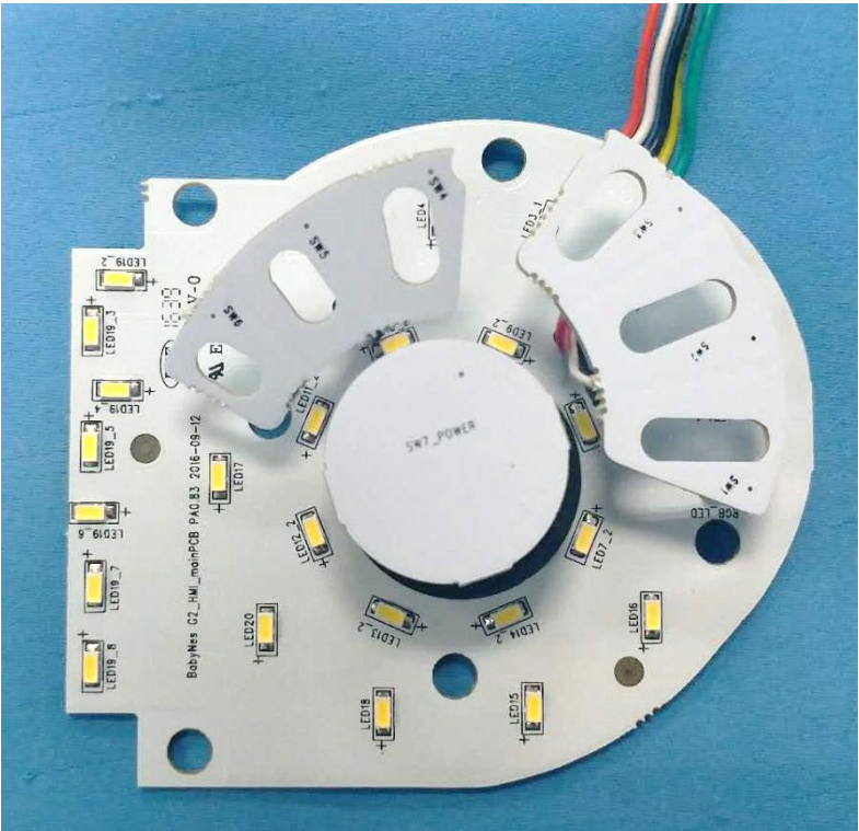
Control board
