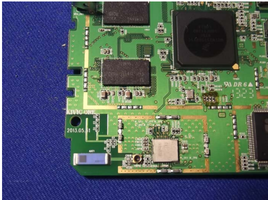
Figure 8 PCB of the Module View
