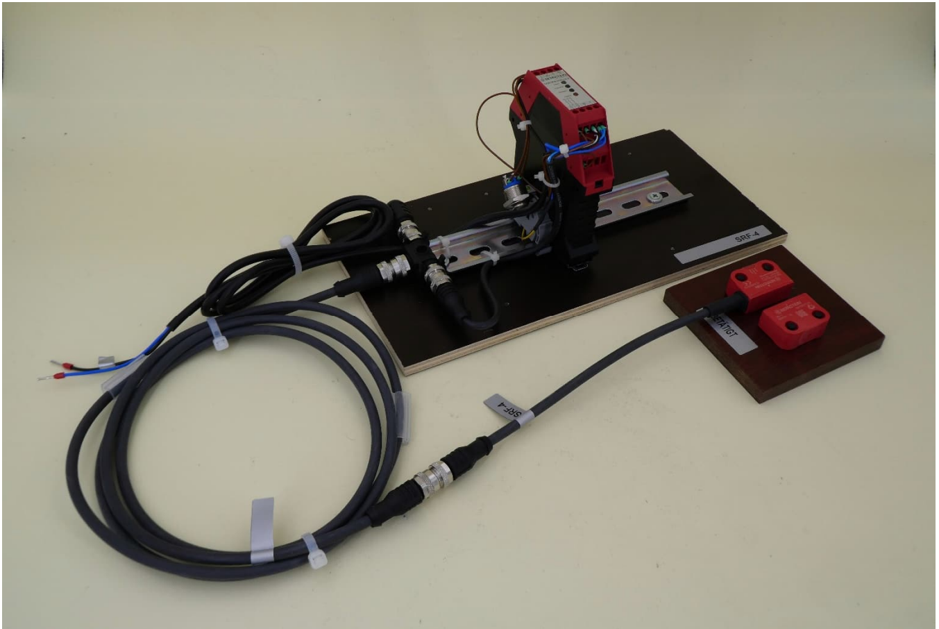
EUT 2 and equipment used for testing – 3D view
