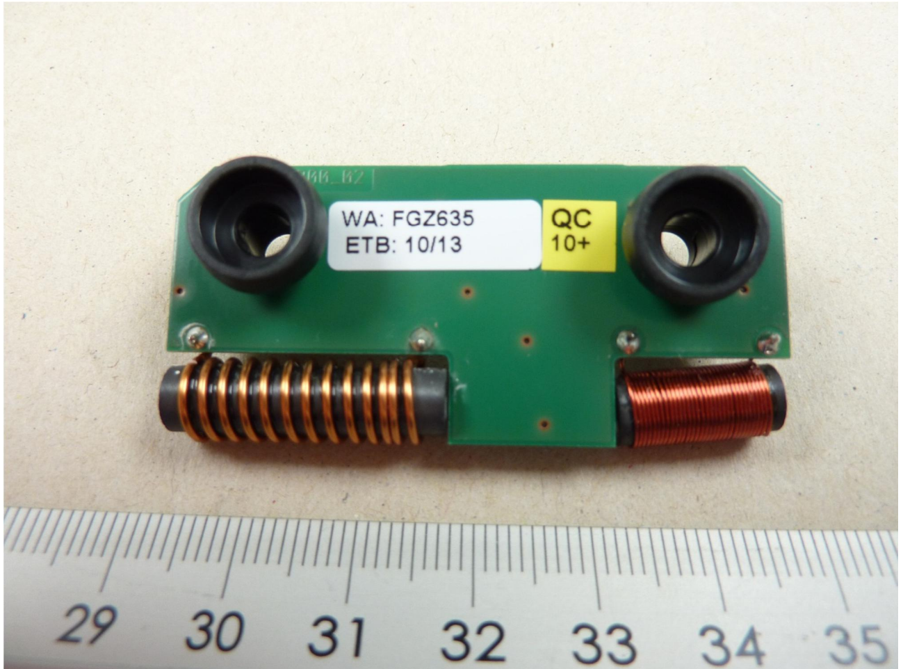
131297eut9.JPG: Transponder, rear view
