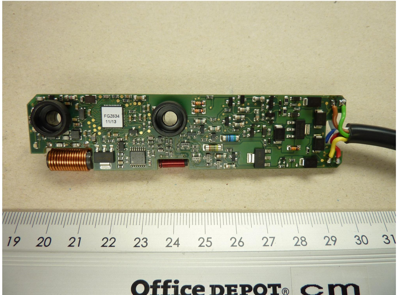
131297eut6.JPG: Transmitter, front view
