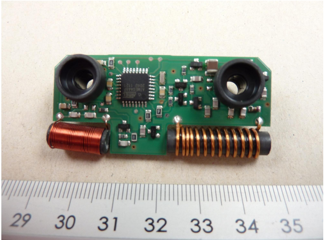
131297eut8.JPG: Transponder, front view
