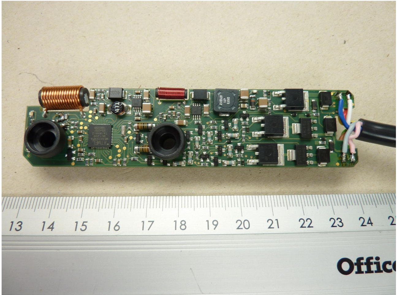
131297eut7.JPG: Transmitter, rear view
