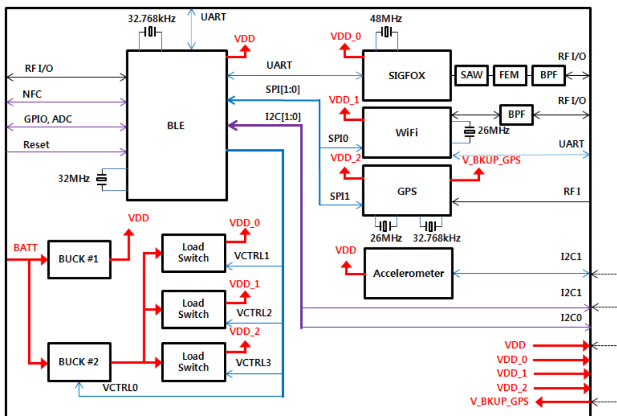
Figure 1-1 WSSFM20R2 block diagram and System Interface
