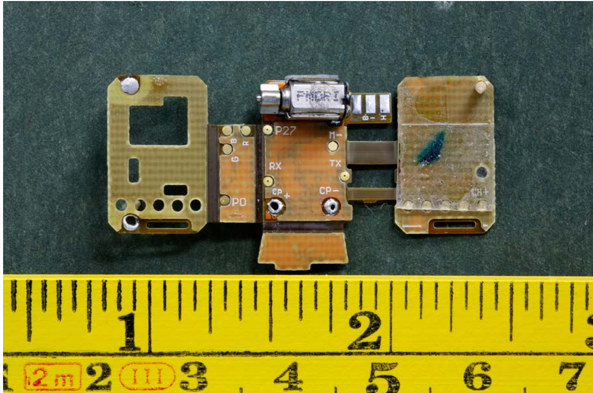
PCB rear
