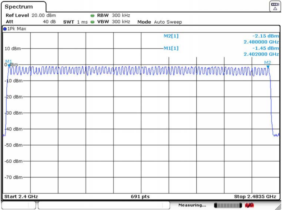
8-DPSK Hopping On
