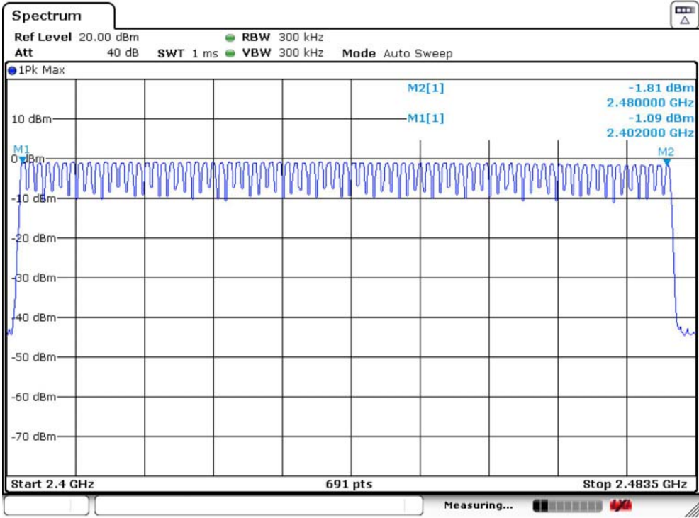
GFSK Hopping On
